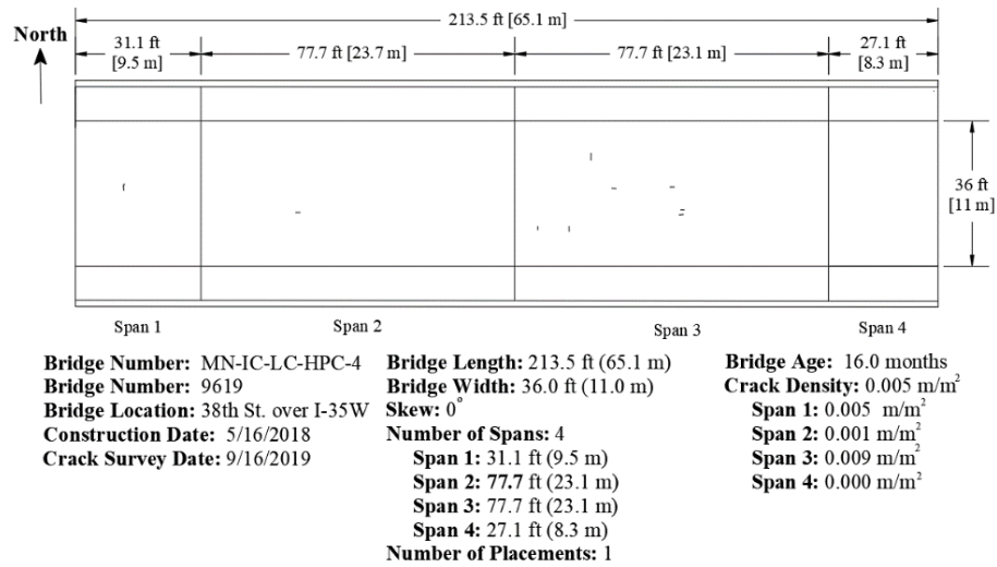
Figure E.13: Crack Map for MN-IC-LC-HPC-4 (Survey 1)
