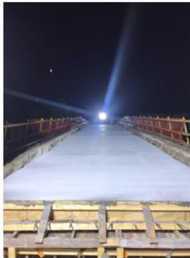
Figure 2.14: The Application of the Curing Compound on the Bridge Deck
