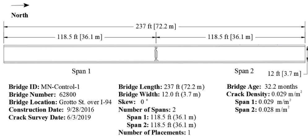
Figure E.6: Crack Map for MN-Control-1 (Survey 3)
