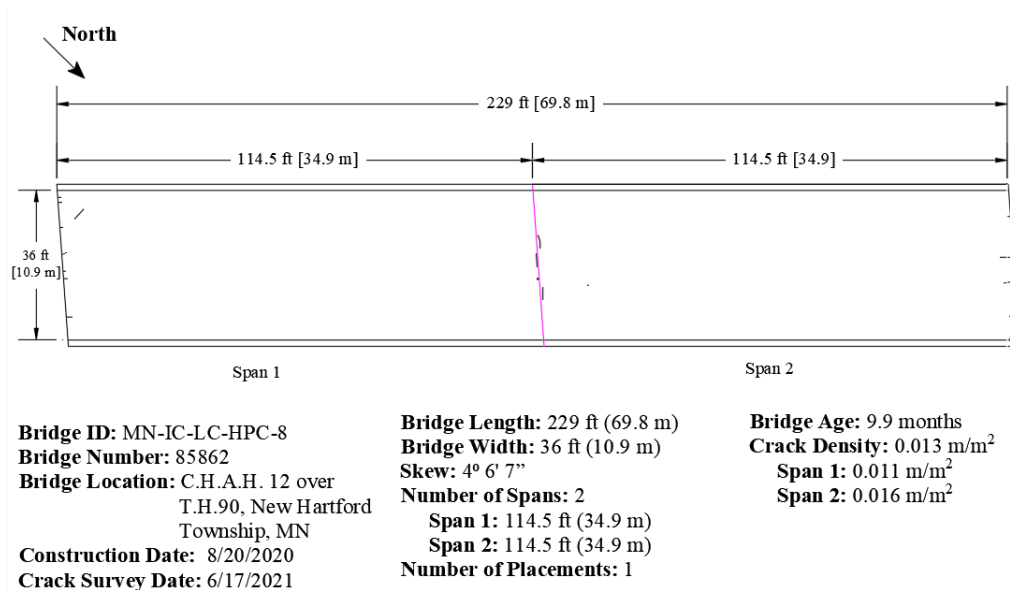
Figure 3.24: Crack Map for MN-IC-LC-HPC-8 (Survey 1)
