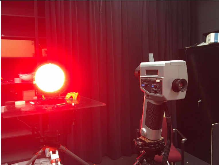
Figure 2 Lab measurement of the signal lens surface luminance using the code recommended method.
