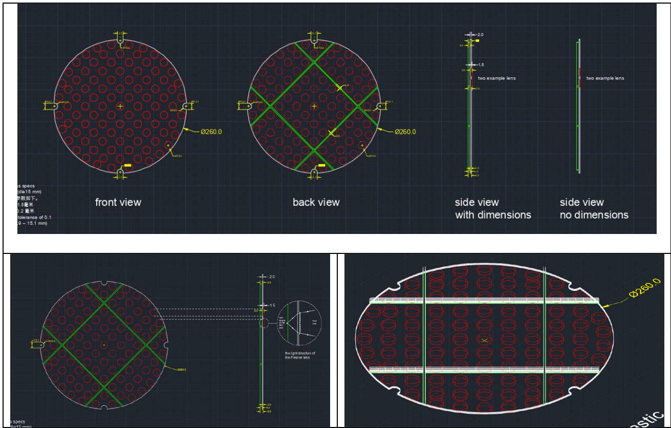
Figure 2 Improved design of the new fresnel disc with 96 small fresnel lenses integrated on it
