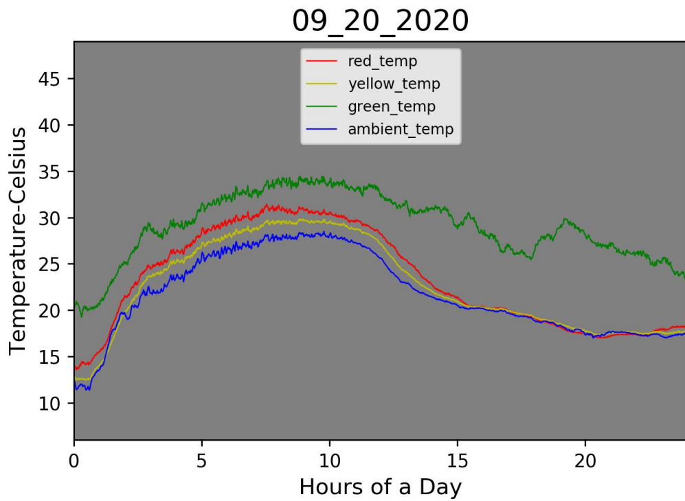
Figure 4 Lawrence field test data during the hottest days in summer 2020 and winter 2019-2020, showing the performance of the red, yellow, and green signal lights under different weather conditions.
