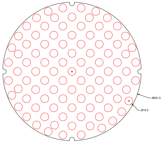
New design of the single lens disc with 96 fresnel lenses embeded on it
