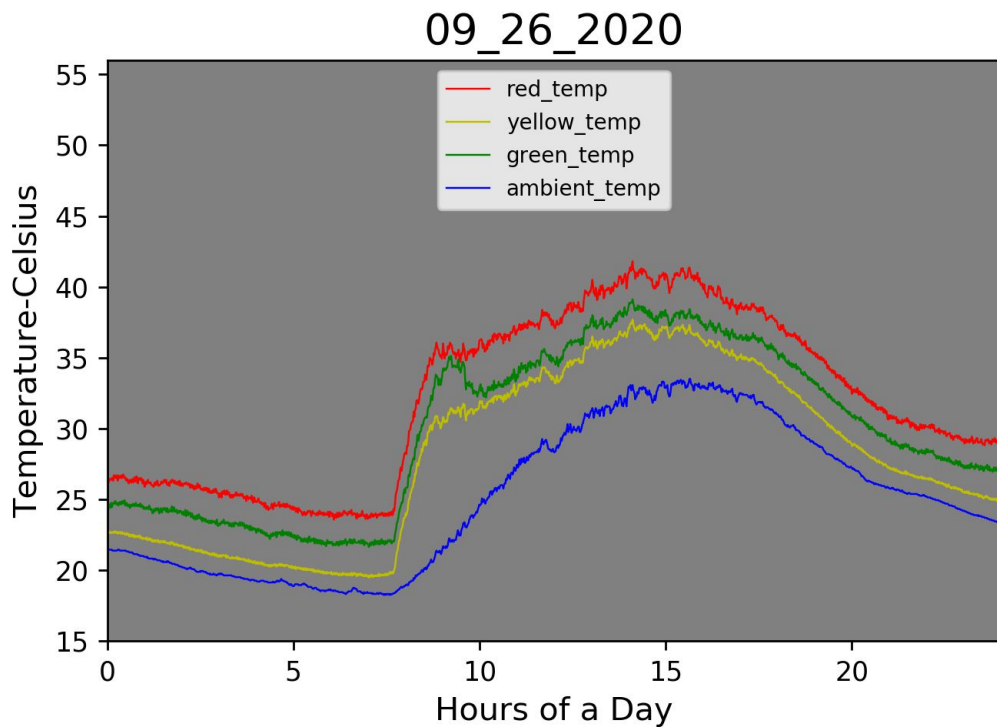
Figure 3 Roof test data during the hottest days (July 7, 18, 24, Aug. 8, 23, 25, 28, Sept. 6, 17, 26) in summer 2020, showing the performance of the red, yellow, and green signal lights under different weather conditions.
