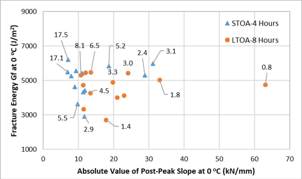
Figure 22. Fracture Energy and Post Peak Slope for all mixture combinations at 0 °C and 0.5 mm/min
