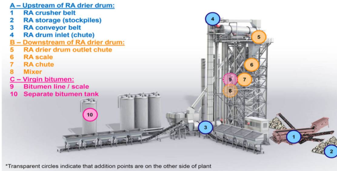
Figure 6.1 Schematic representation of potential rejuvenator dosing locations (Zaumanis, Cavalli, & Poulikakos, 2020).
