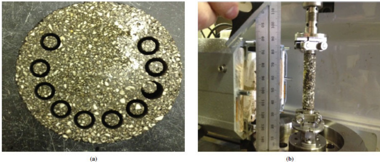
Figure 4.1: Preparation process for FAM specimens including (a) coring locations of cut gyratory-compact specimen and (b) test setup (Kanna, Ozer, & Al-Qadi, 2014).
