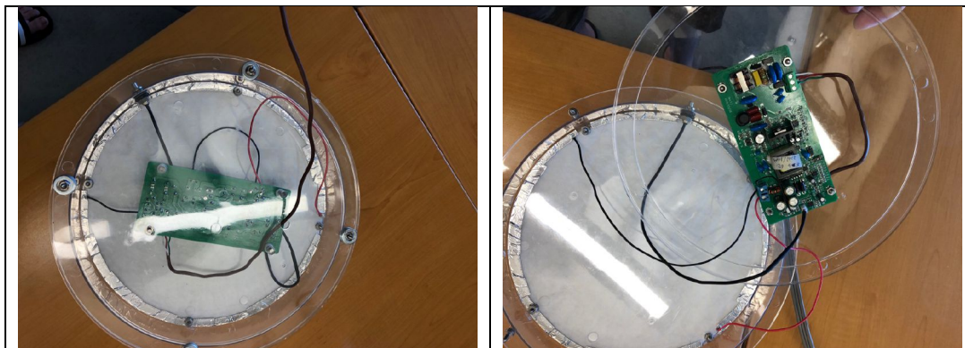
Figure 2 Improved signal housing fitted with the second generation of LED drivers.
