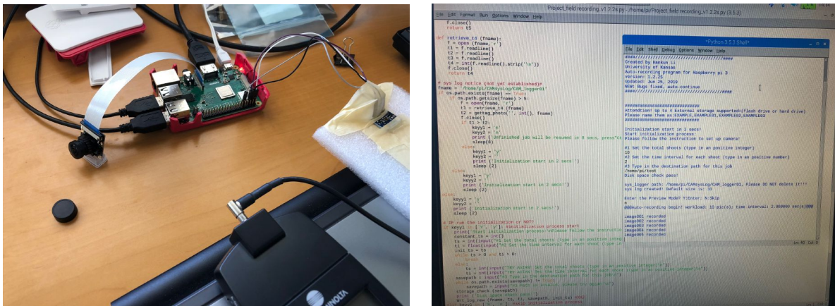
Figure 4 Custom design and lab testing of the monitoring cameras – Raspberry 3 B+ motherboard and accessories, to be used in field tests over 1-2 years without interruption.
