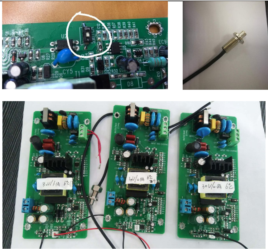
Figure 1 The second generation of LED drivers with all improvements
