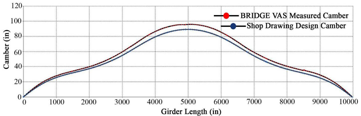
Figure 35. BRIDGE VAS Camber Measurement of a Six-Segment Girder Line Total Length of About 830 ft (BRIDGE VAS Measured, top line; Shop Design, lower line)
