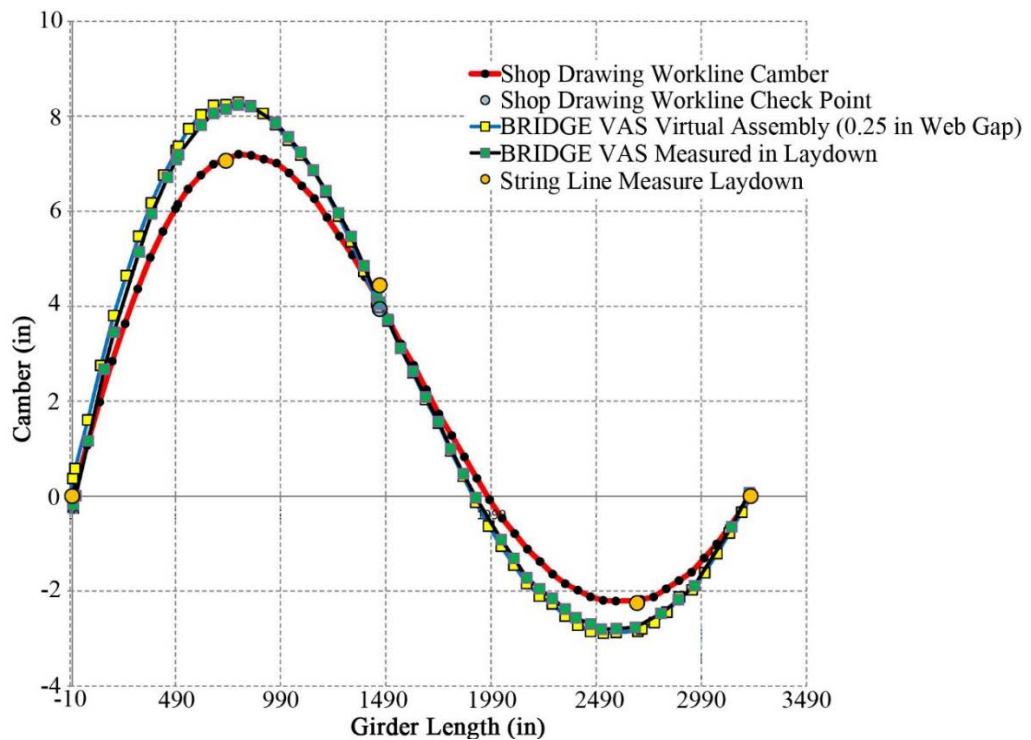
Figure 51. Combined Camber Diagram Comparing Actual Laydown BRIDGE VAS Measurement to BRIDGE VAS Virtual Assembly
