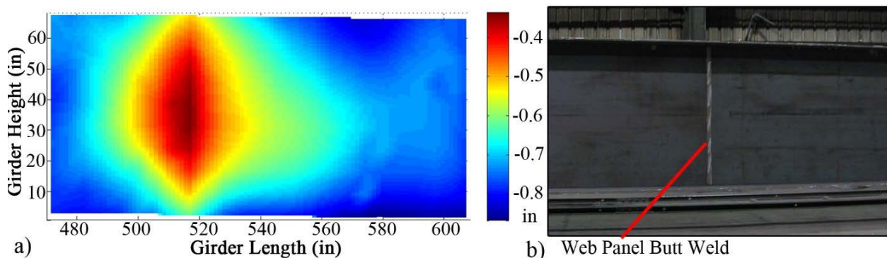
Figure 41. BRIDGE VAS Measurements Showing a) Web Panel Deformations at a Web Plate Butt Splice and b) a Photograph of the Butt Weld
