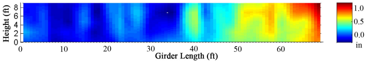
Figure 43. Web Panel Deformations of Tub Girder Far Side Web
