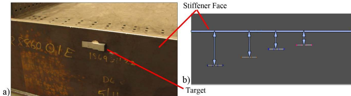
Figure 49. Validator Target Measurement at 157 ft Showing a) the Target on a Stiffener and b) the Measurement of the Target Steps
