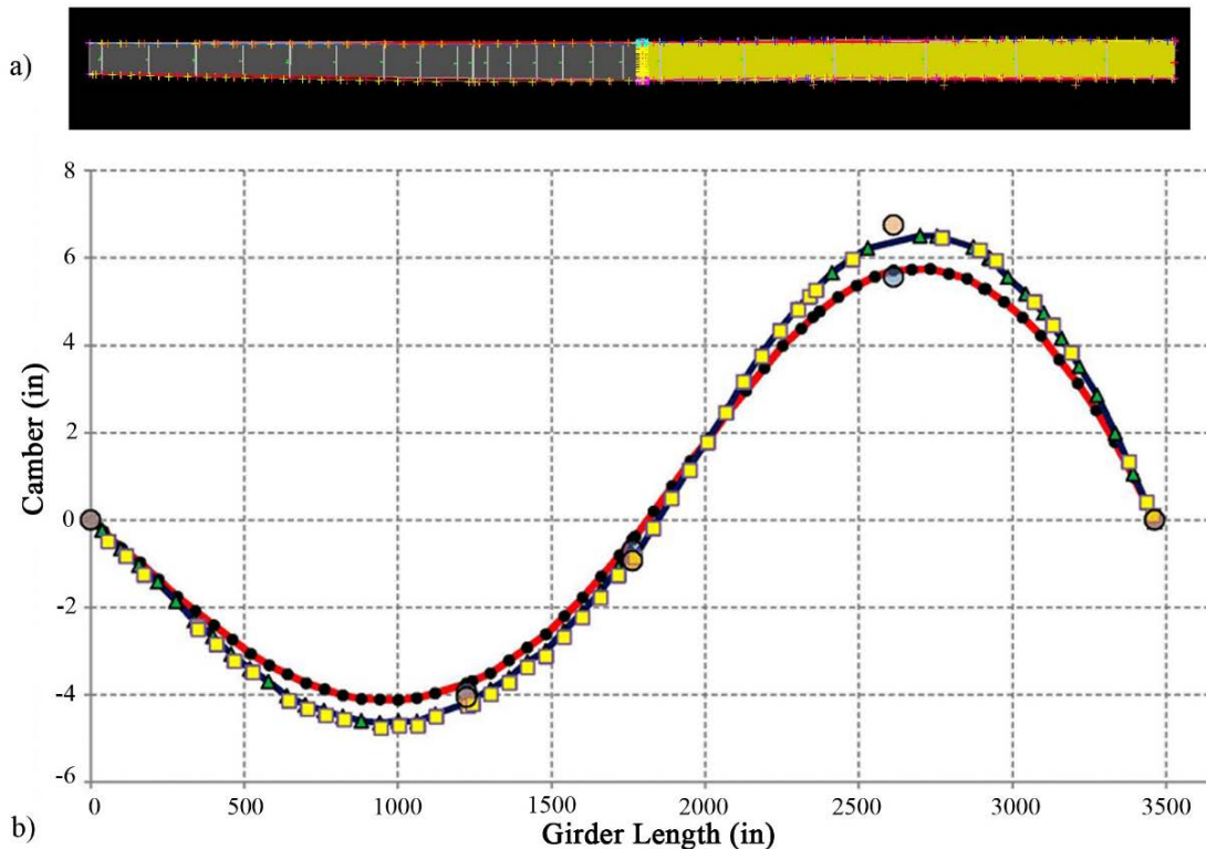
Figure 3. Bridge VAS Software Manipulating a) Individual Girder Pair Measurements Based on b) Optimized Virtual Assembly Based on Combined Camber
