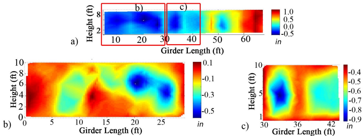
Figure 44. Close-Up View of Tub Girder Near Side Web Panel Deformations Showing a) Entire Web Panel and b) Close-Up Section from 0 to 30 ft and c) Close-Up Section from 30 to 42 ft
