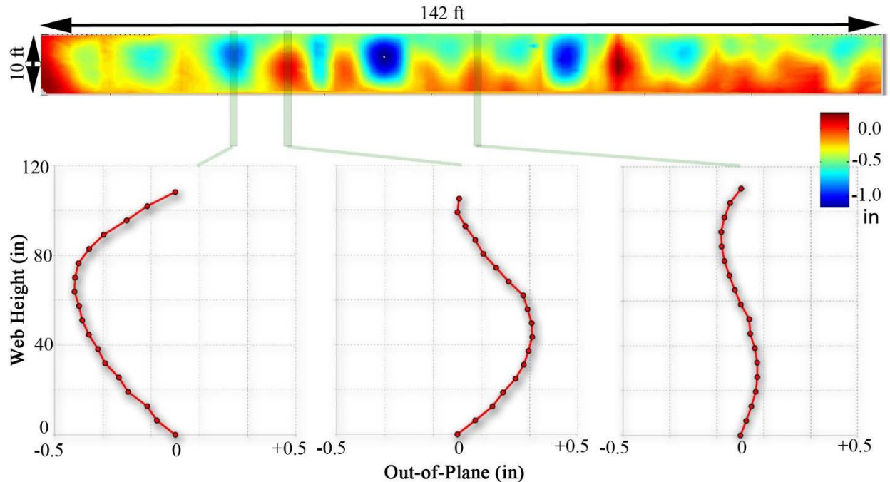
Figure 40. Web Panel Deformation Measurements Shown for a Very Large (142 × 10 ft) Girder Web
