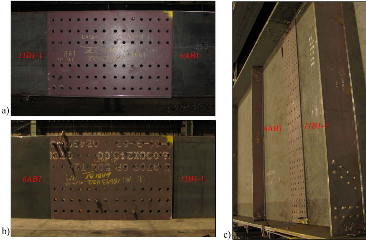
Figure 56. BRIDGE VAS Detailed Splice Plates Fit-Up in Girder Laydown Showing a) Top Flange, b) Bottom Flange, and c) Web Plates
