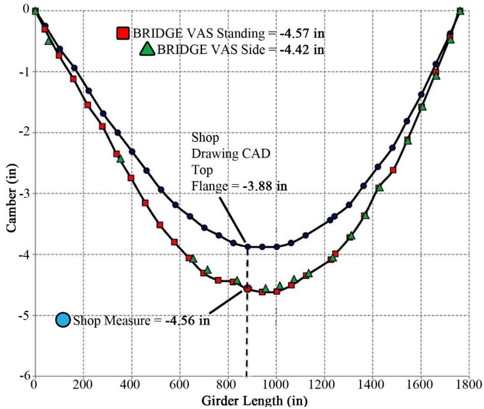
Figure 33. Camber Measurements on Girder 6AB1 Comparing Standing and Laydown Measurements
