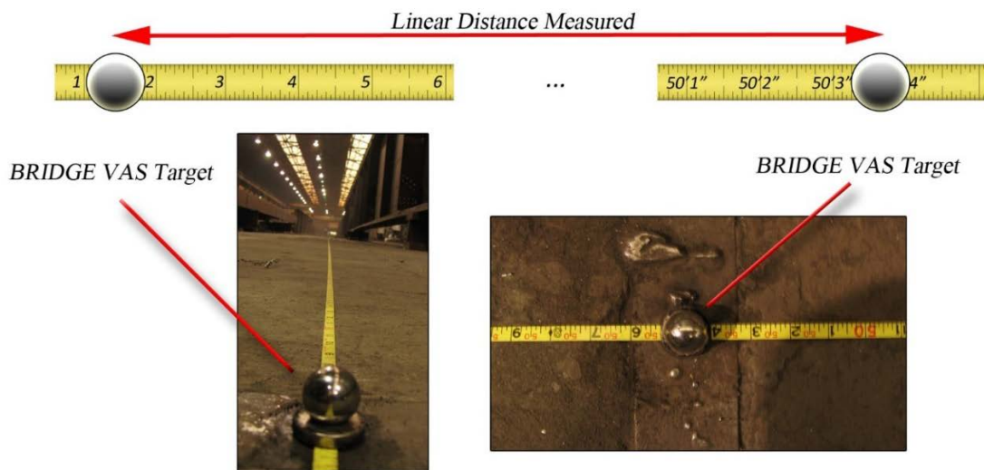
Figure 27. Certified Tape Measured Over About 50 ft on Shop Floor
