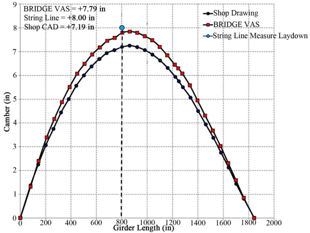
Figure A8. Girder 17B2-2 Top Flange Camber
