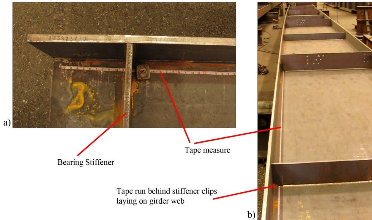
Figure 24. Conventional Length Measurements Using Tape Measure Showing a) Measurements Around a Stiffener and b) Measurements Behind Stiffener Clips
