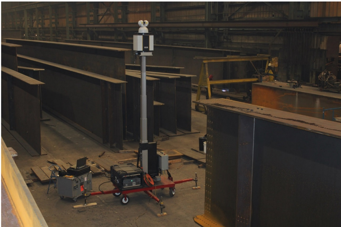
Figure 11. BRIDGE VAS Measuring a Steel Girder in a Fabrication Shop
