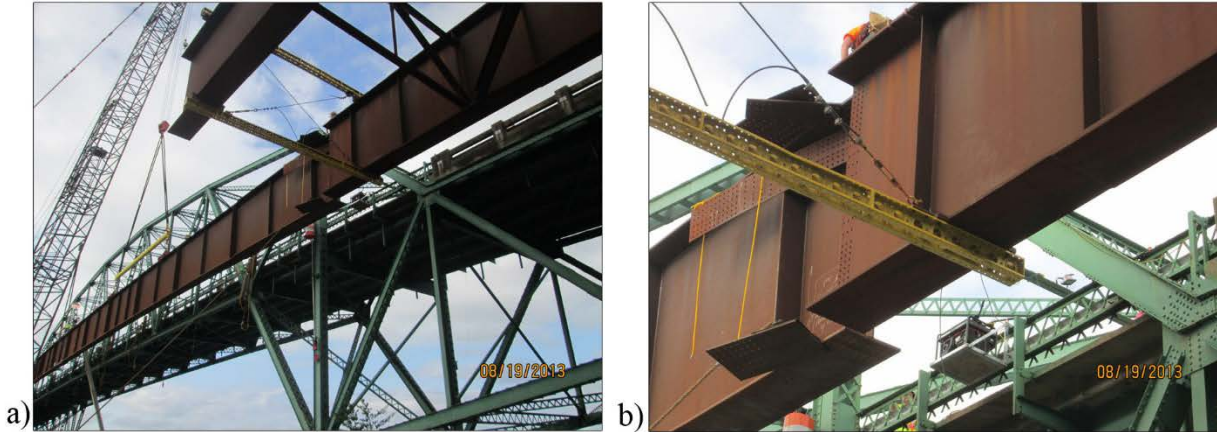
Figure 58. Erection of a) Line 1 Splice 2, Girder 6AB1 to 11B1-1 and b) Close-Up of Splice (Photos provided by H. Pate, Tennessee Department of Transportation)
