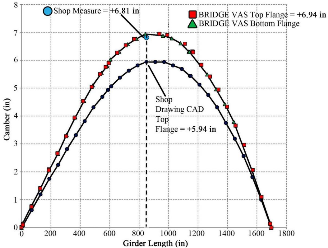
Figure 34. Girder Camber for 12B2-1 Showing Both Top Flange and Bottom Flange Camber
