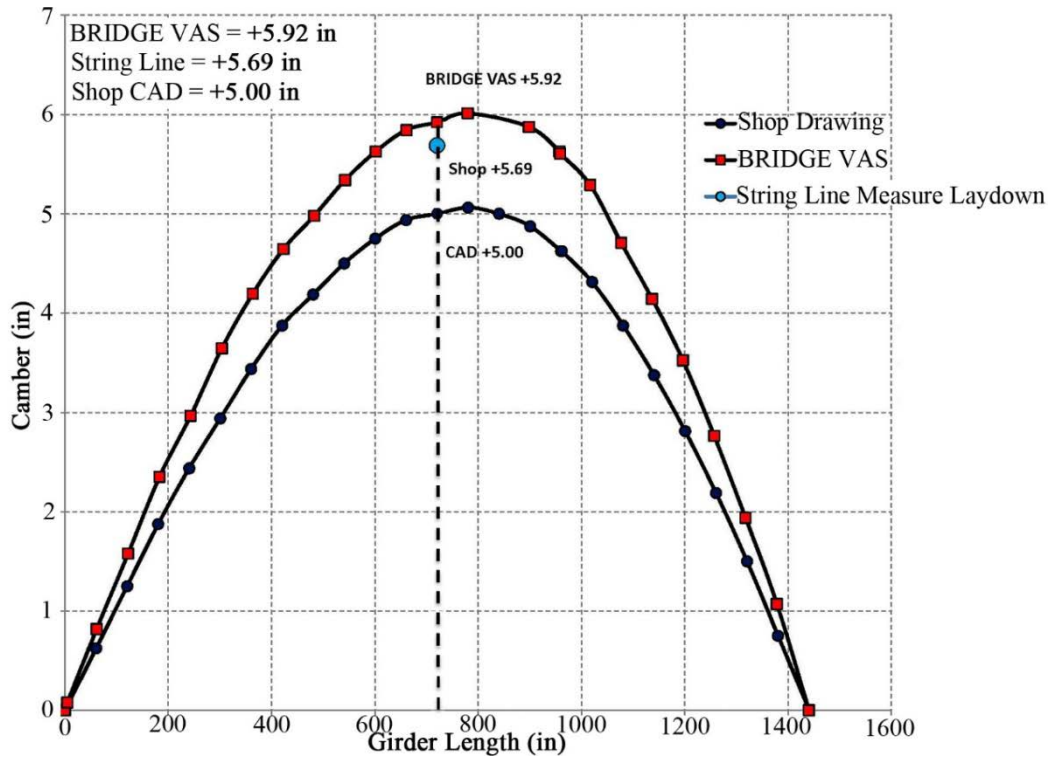
Figure A12. Girder 27C2 Top Flange Camber
