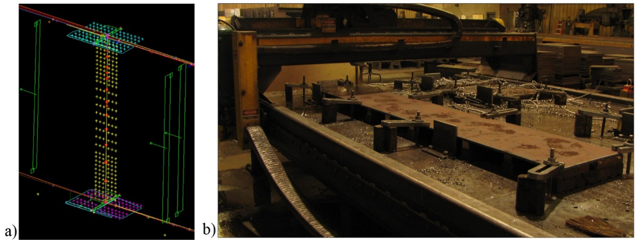
Figure 20. Virtual assembly of Girder Pair Output Showing a) Close-Up of Splice with Measured Hole Locations and b) CNC Drilling Machine Making Custom Splice Plate from BRIDGE VAS Output
