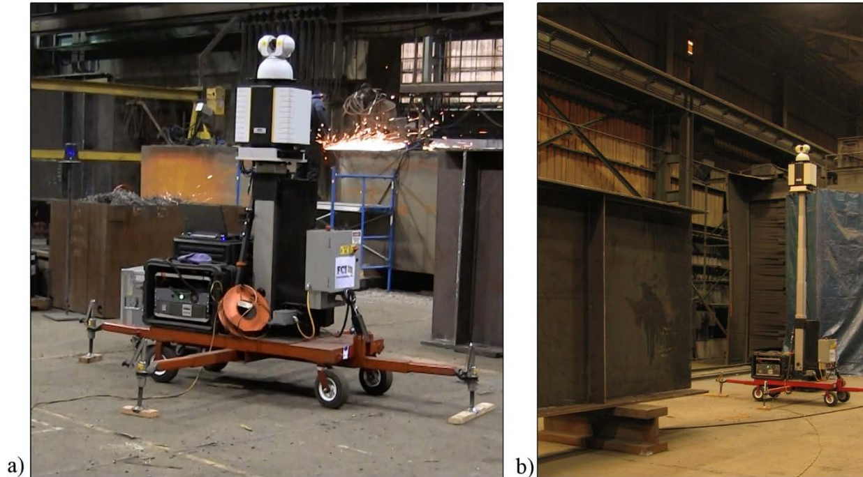
Figure 12. System Operates in Normal Shop Environment Around Existing Processes; Such as a) Grinding and b) Blast Cleaning
