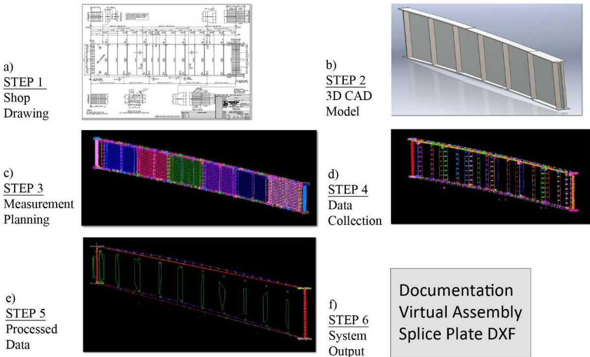
Figure 17. System Processes Steps
