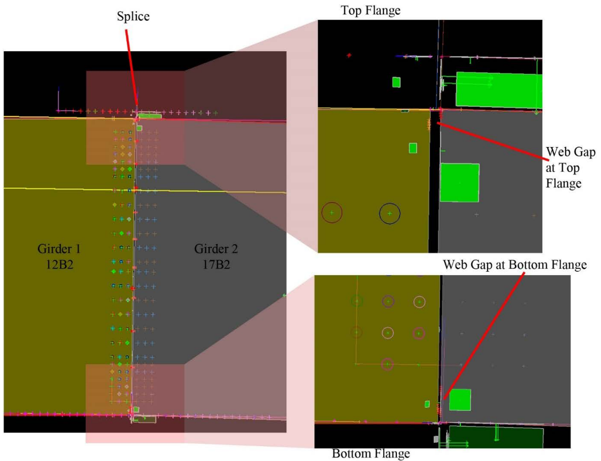
Figure 47. Virtual Assembly of a Girder Pair Showing Details of the Splice Fit-Up
