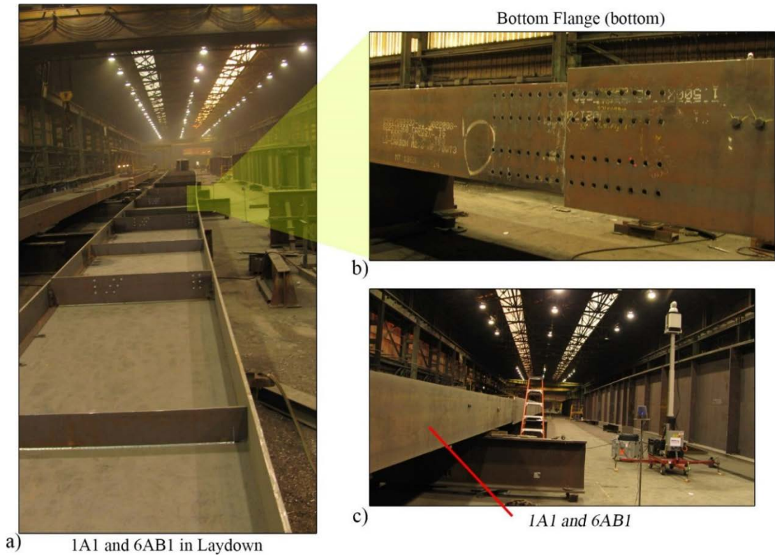
Figure 50. Laydown Measurement of Girders for Comparison to Virtual Assembly Showing a) the Girder Pair and b) a Close-Up of the Girder Pair Splice Bottom Flange and c) the Measurement Location of the BRIDGE VAS for Laydown Measurements
