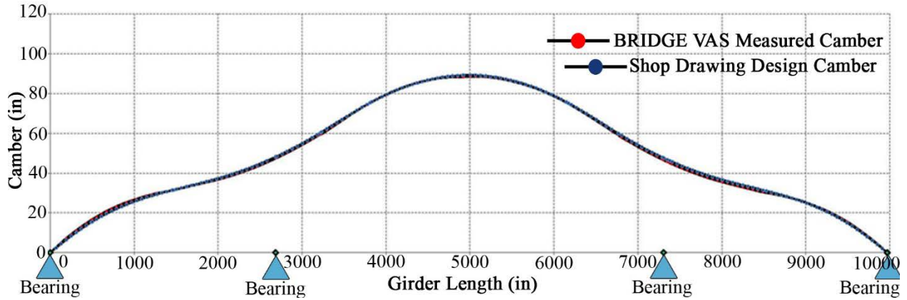
Figure 46. Line Camber Data Comparing Measured Values to Shop Nominal Data for Girder Line 2
