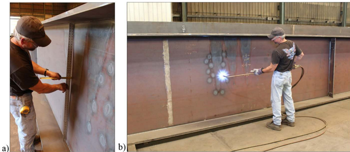
Figure 39. Reworking of Girder Web Showing a) Conventional Straight Edge Web Panel Measurement and b) Heating of Web to Change Shape
