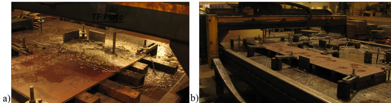
Figure 55. Fabrication of BRIDGE VAS Detailed: a) Top Flange Plate and b) Web Plate
