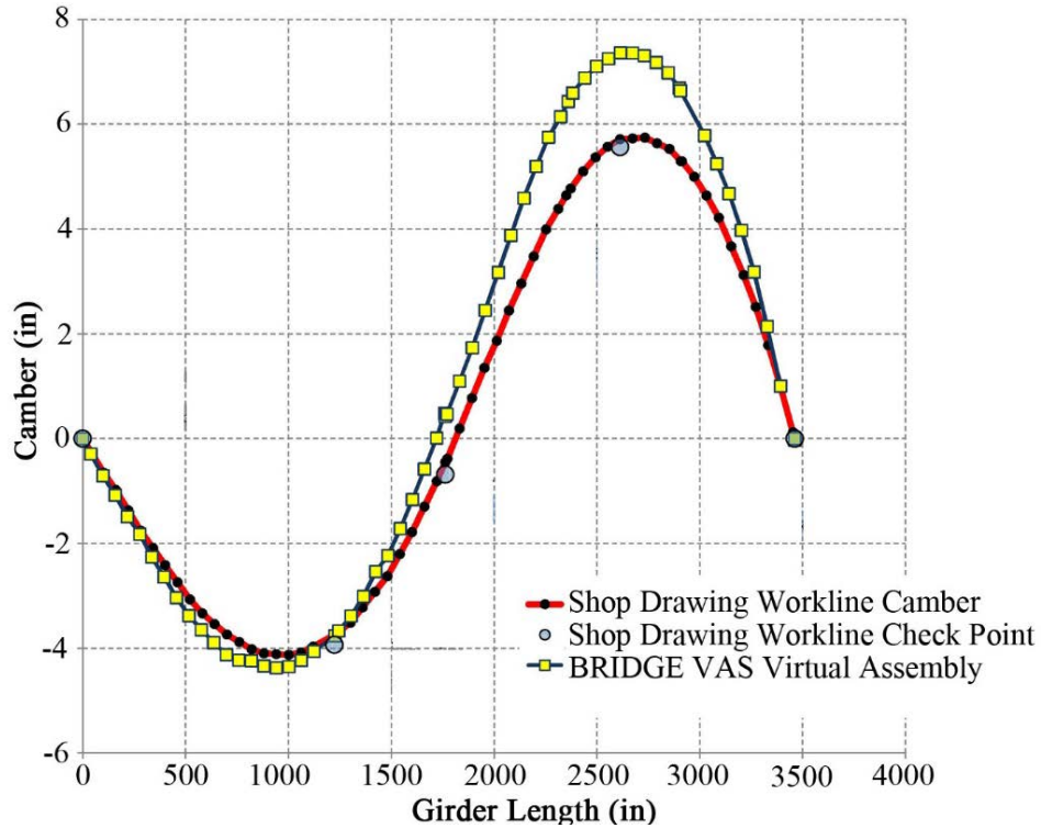
Figure 54. Combined Camber Diagram of Girder Pair for Virtual Assembly of 6AB1 and 11B1-1
