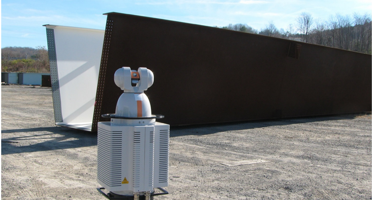
Figure 13. BRIDGE VAS Measures All Types of Fabricated Girders Including Large Tubs
