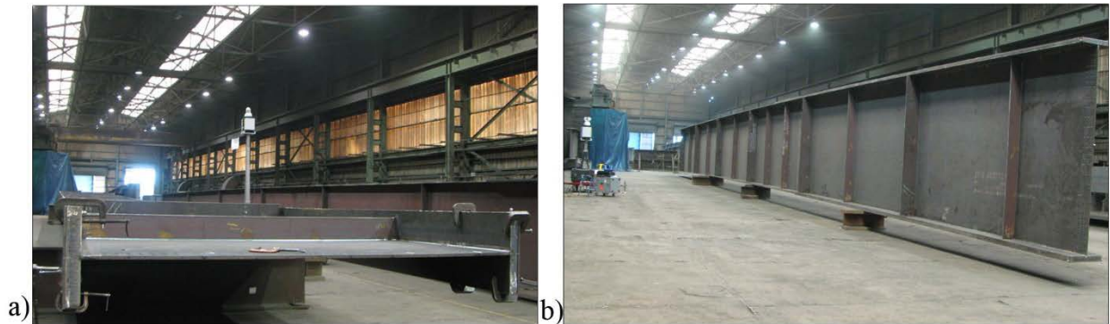
Figure 31. Girder 11B1-1 Camber Measurements with a) Girder on Side and b) Girder in Standing Position
