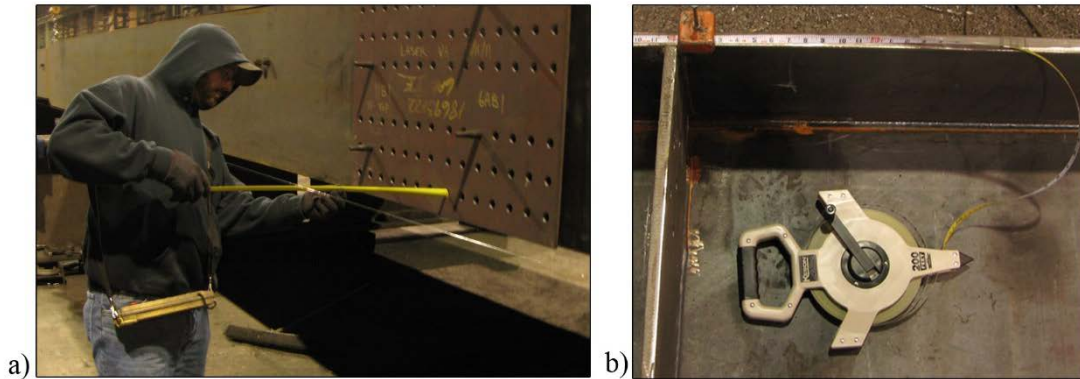
Figure 4. Conventional Measurements a) With Rulers/String Line and b) Tape Measures
