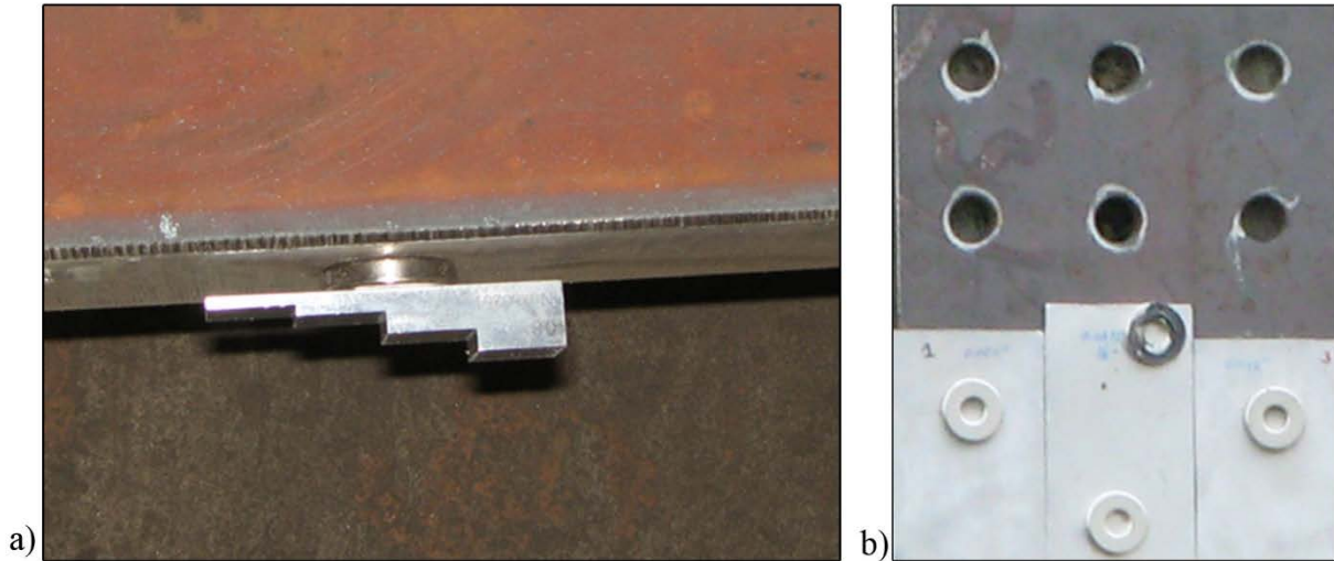
Figure 16. Validator Targets with a) Precision Steps and b) Hole and Step Patterns
