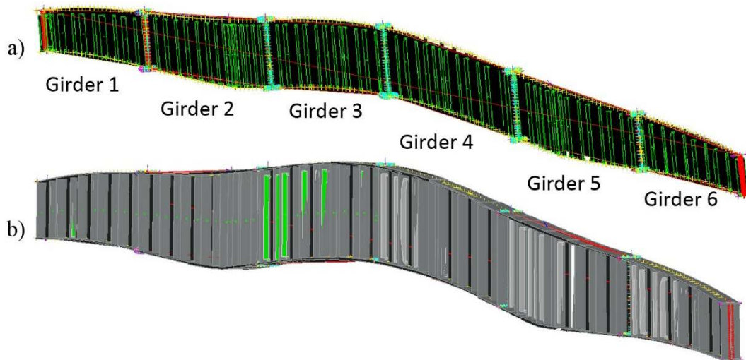
Figure 45. Virtual Assembly of an Entire Girder Line: a) Measured Data and b) Measured Data with 3D Model
