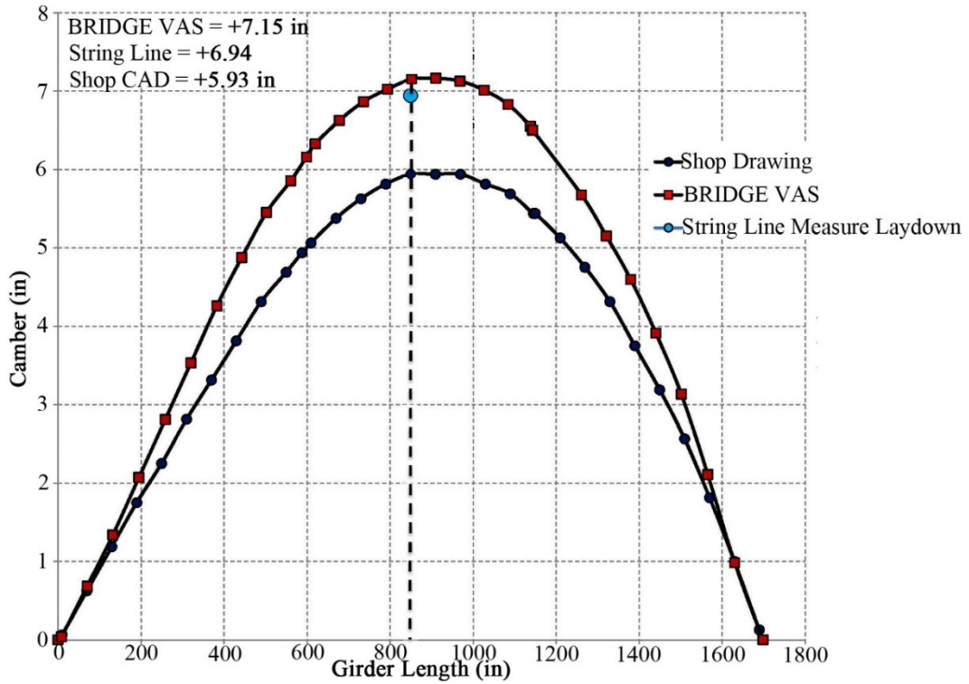
Figure A5. Girder 11B1-1 Top Flange Camber
