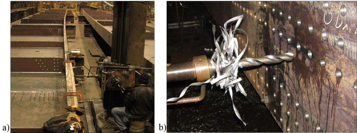
Figure 1. Match-Drilling: a) Girders Lay on Their Side and b) Web and Flanges Drilled Using Template
