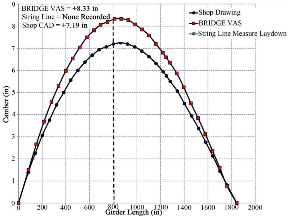
Figure A7. Girder 16B1-2 Top Flange Camber
