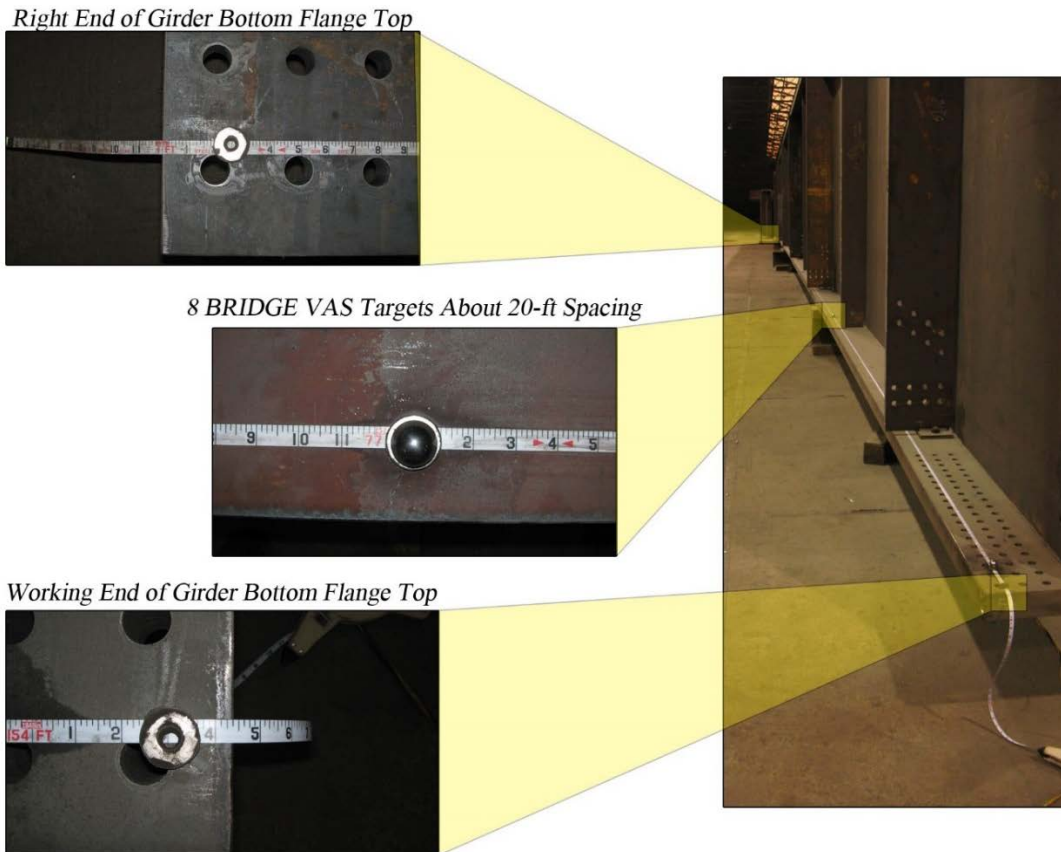
Figure 29. 200-ft Tape Measure Placed on Top of Girder Bottom Flange
