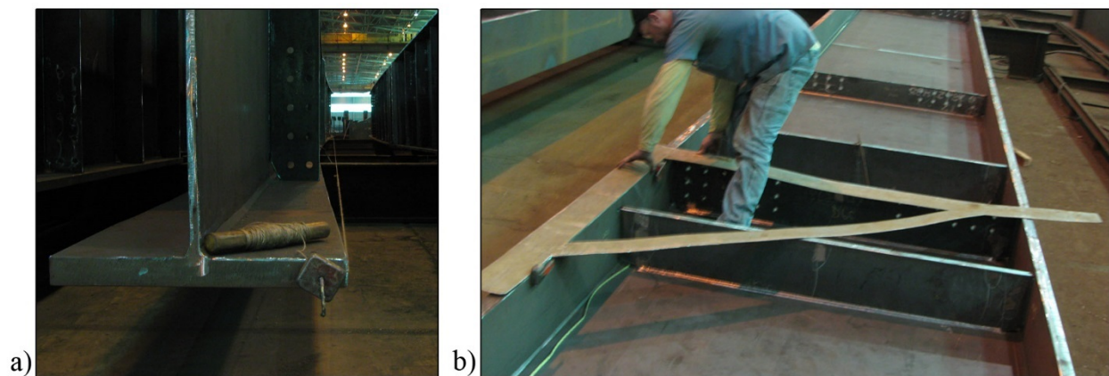
Figure 21. Conventional Measurement Tools Showing a) String Lines and b) Straight-Edges
