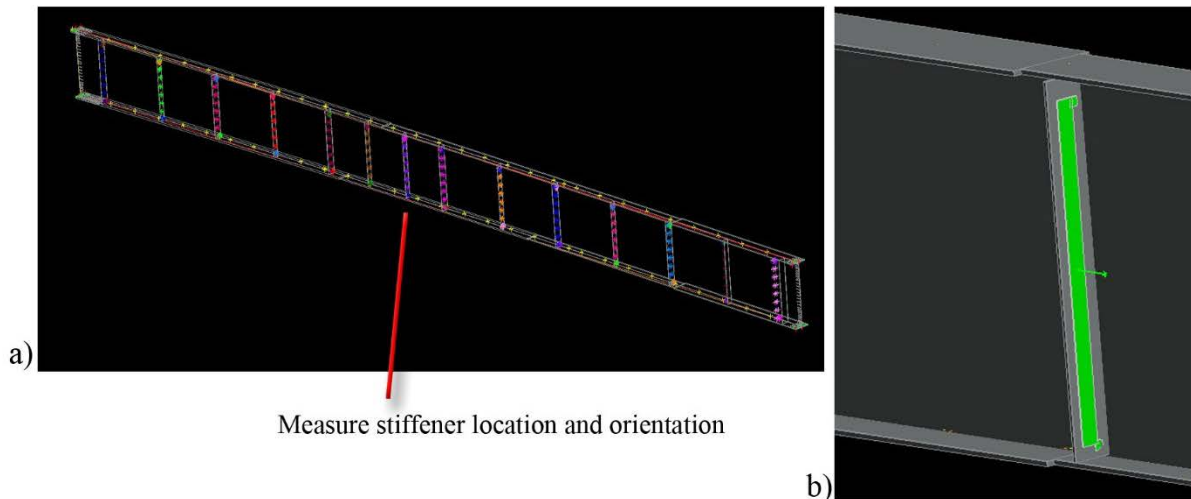
Figure 38. Measurement of Girder Stiffener Location and Orientation Showing a) Multiple Stiffeners Along Length of Girder and b) Close-Up of Stiffener Measurement (Green) Overlaid on Ideal 3D CAD Model
