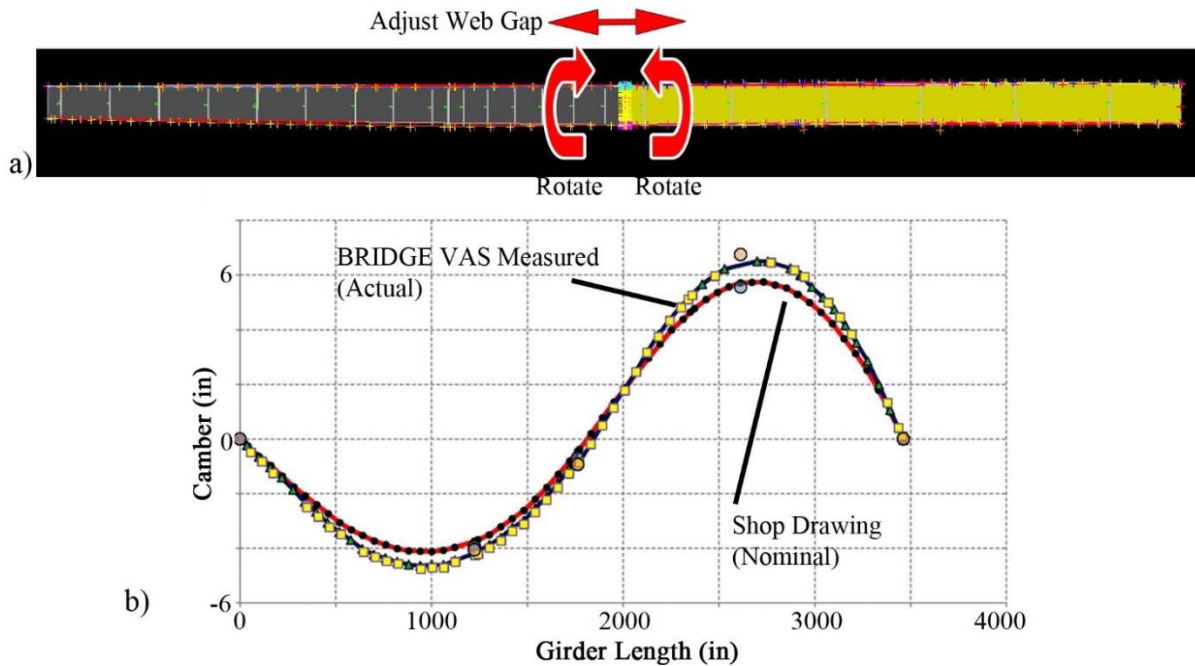
Figure 19. Virtual Assembly of Girder Pair with a) Measured Data from Two Girders Showing How Girder Are Virtually Positioned Based on the b) Combined Camber Shop Drawing Criteria
