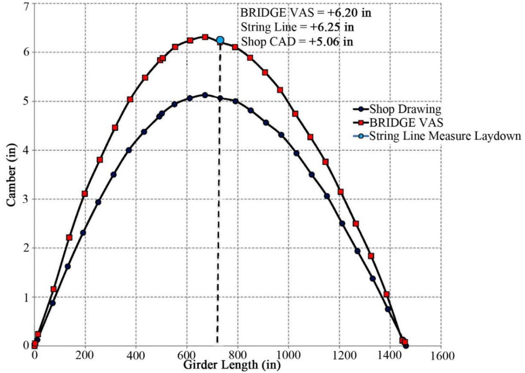
Figure A1. Girder 1A1 Top Flange Camber
