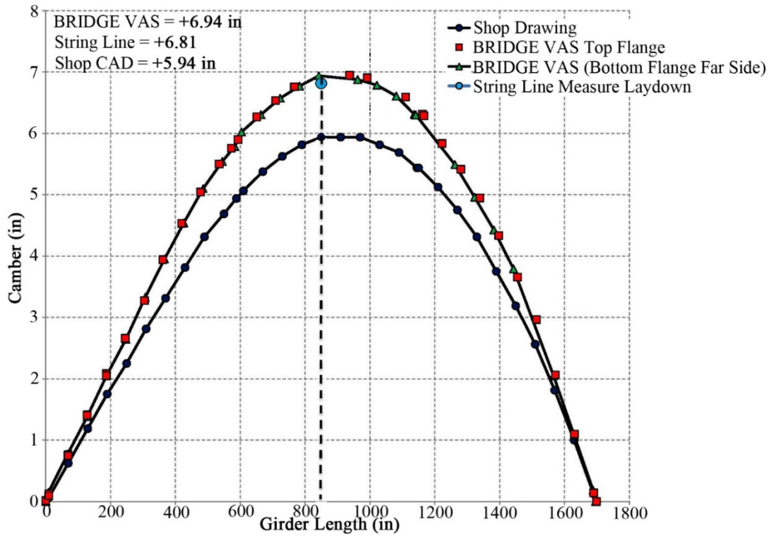
Figure A6. Girder 12B2-1 Top and Bottom Flange Camber
