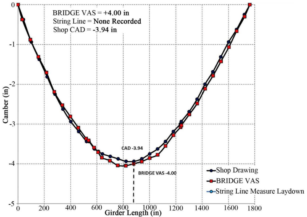
Figure A9. Girder 21BC1 Top Flange Camber
