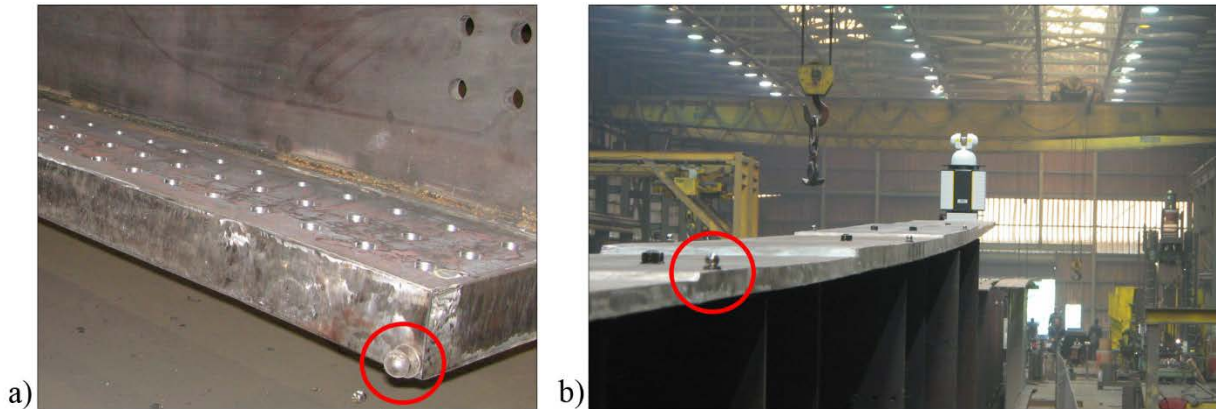
Figure 15. Magnetic Mounted Targets a) for Alignment to CAD and b) for System Repositioning
