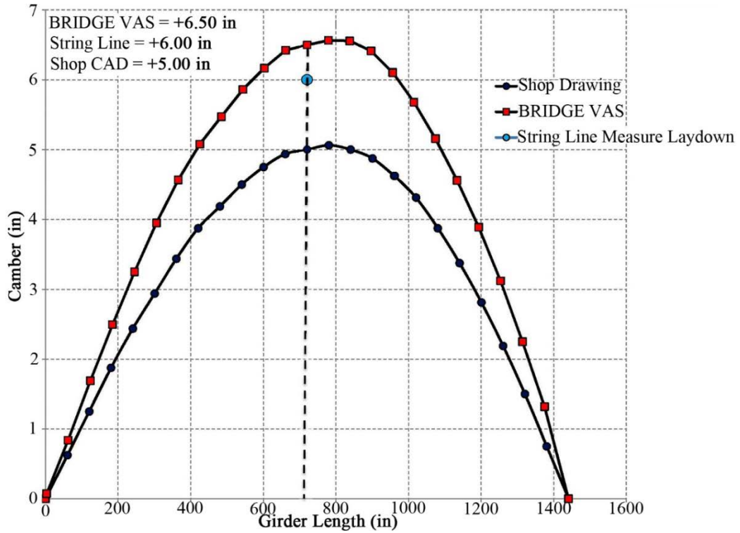
Figure A11. Girder 26C1 Top Flange Camber
