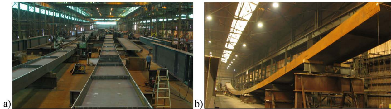
Figure 2. Laydown Process in a Typical Fabrication Shop Requires Substantial Floor Space for Both a) Straight Girders and b) Curved Girders
