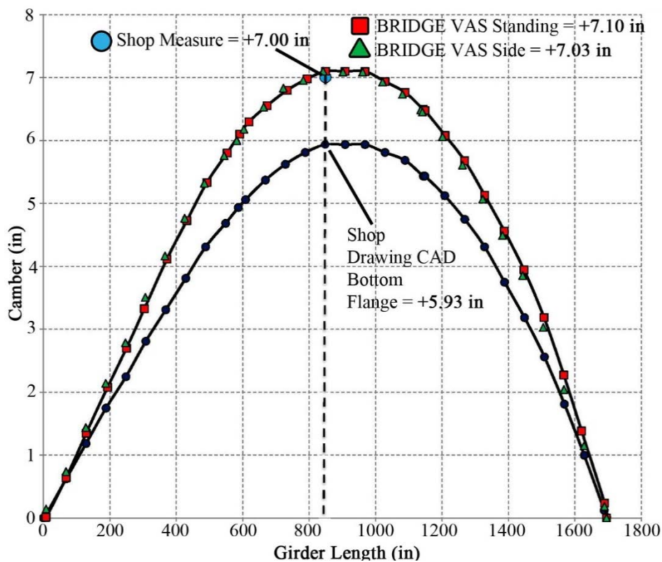
Figure 32. Camber Measurements on Girder 11B1-1 Comparing Standing and Laydown Measurements
