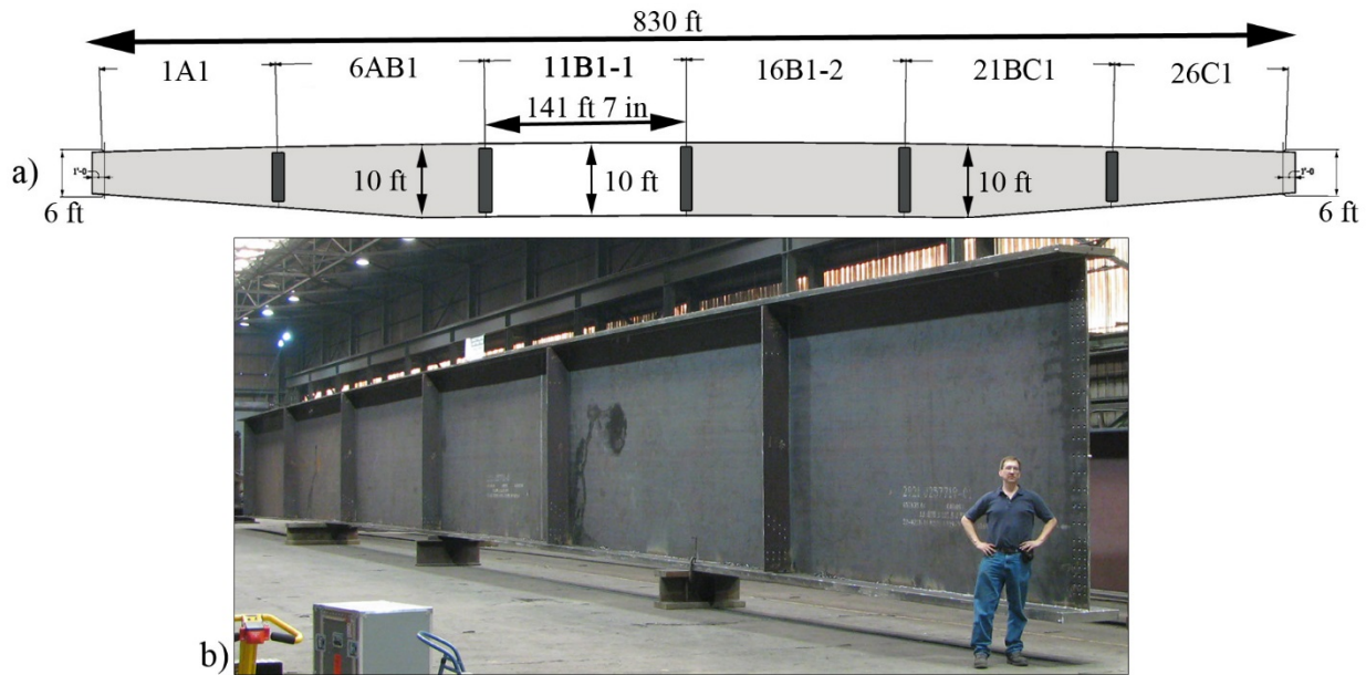
Figure 8. Girder Line: Straight with a Linear Taper, Showing a) the Entire Line Drawing and b) Girder 11B1-1 (Length 141 Ft – 7 In, Web Depth 10 Ft)
