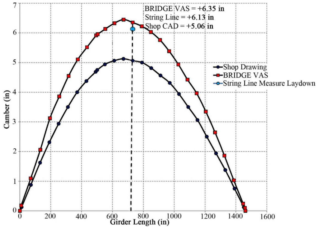
Figure A2. Girder 2A2 Top Flange Camber
