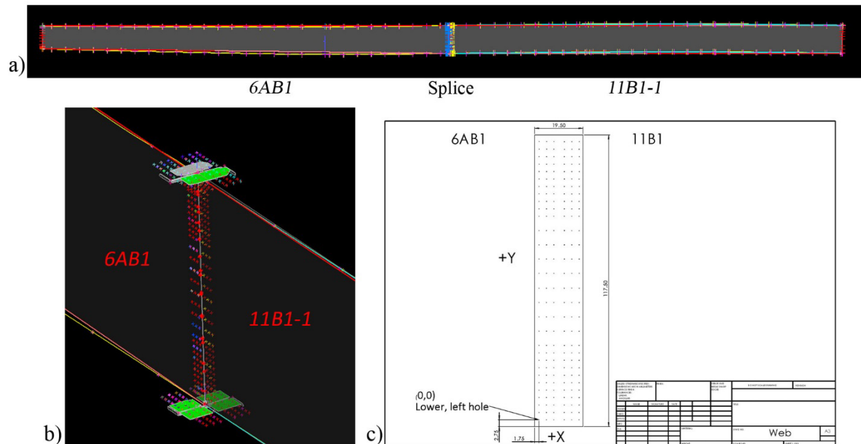
Figure 53. Virtual Assembly of a) Girder Pair 6AB1 to 11B1-1 Showing b) Close-Up of Splice and c) Resulting Custom Splice Web Plate Detail
