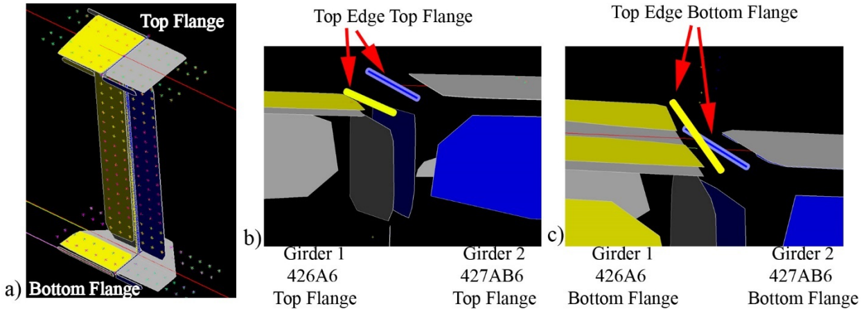
Figure 48. Virtual Assembly Fit-Up Details Showing a) a Splice and b) Close-Up of the Top Flange and c) Close-Up of the Bottom Flange
