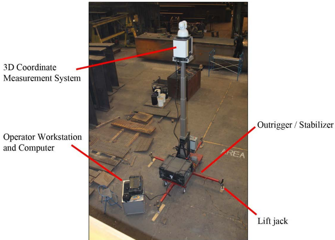
Figure 14. BRIDGE VAS Basic System Components
