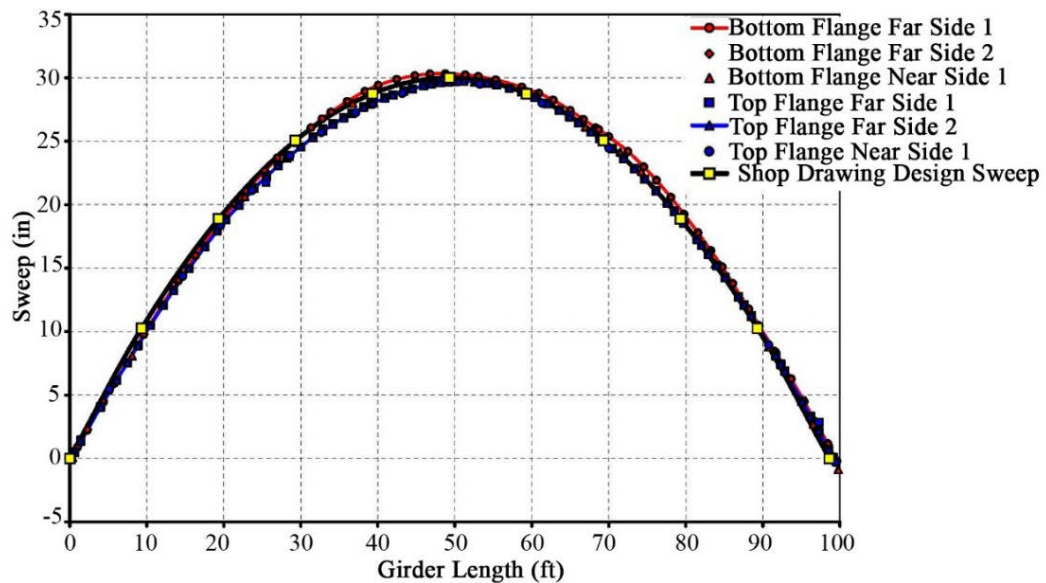
Figure 37. Sweep Measurement of 100 ft Long Curved Girder Showing Shop Drawing Nominal Sweep (Yellow Square) and BRIDGE VAS Measurements at Multiple Locations on the Girder
