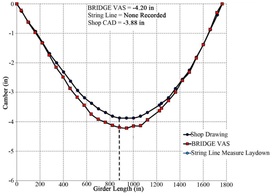
Figure A4. Girder 7AB2 Top Flange Camber
