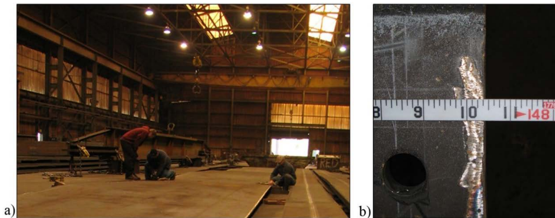
Figure 23. Tape Measurement a) of Flat Plates and b) Showing Measurement of an Irregular Edge
