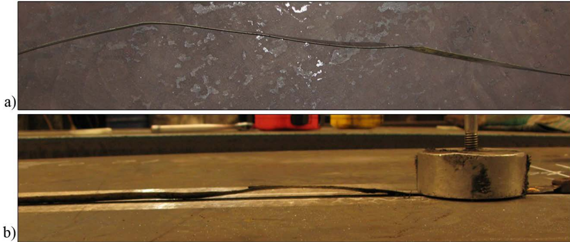
Figure 25. Tape Measure Used on Shop Floor Showing a) Bends and b) Kinks in Metal Tape
