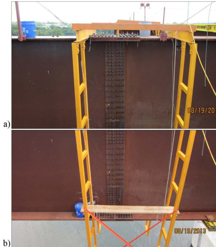
Figure 59. Line 1 Field Splice 2, Girder 6AB1 to 11B1-1, Showing Final Fit-Up of a) Top Flange and Top of Web Plate and b) Bottom of Web Plate and Bottom Flange (Photos provided by H. Pate, Tennessee Department of Transportation)
