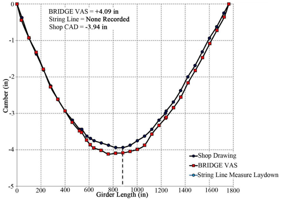
Figure A10. Girder 22BC2 Top Flange Camber
