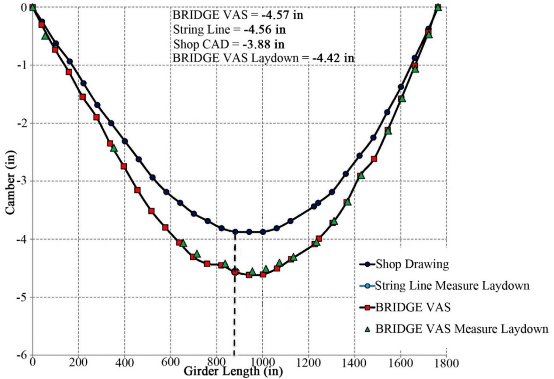
Figure A3. Girder 6AB1 Top Flange Camber
