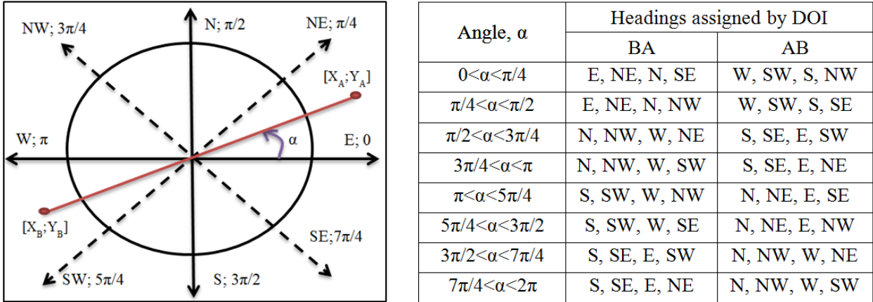
FIGURE 10 DOI Heading Assignment.
