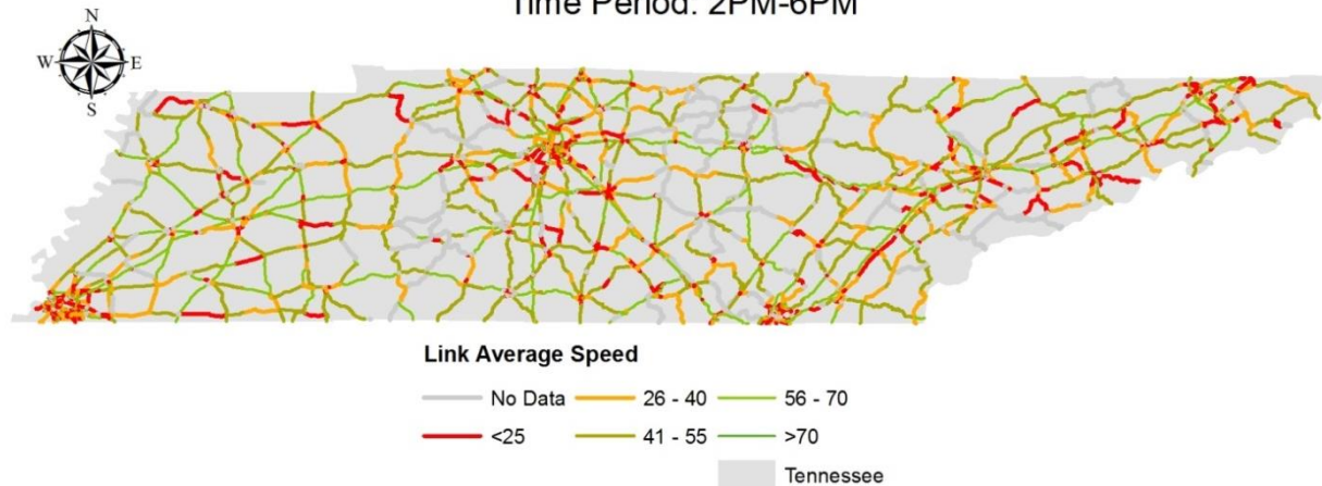
FIGURE A-4d Link Average Speeds, May 15th - 17th, PM Period.
