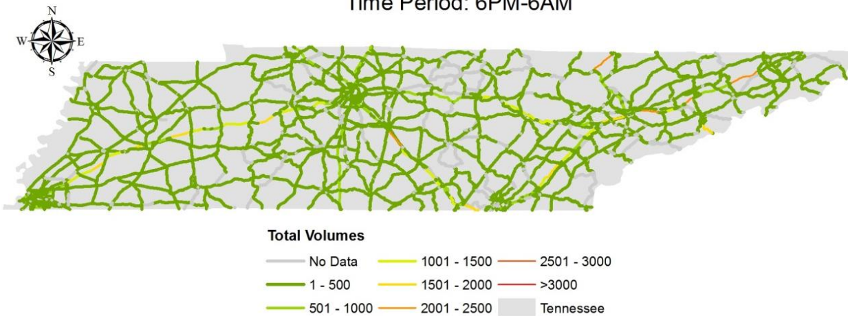
FIGURE B-14b Total Volumes, August 14 th - 16 th , OP Period.
