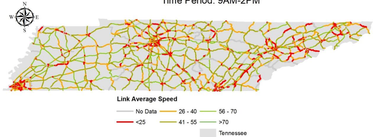
FIGURE A-8b Average Speeds, September 18 th - 20 th , MD Period.
