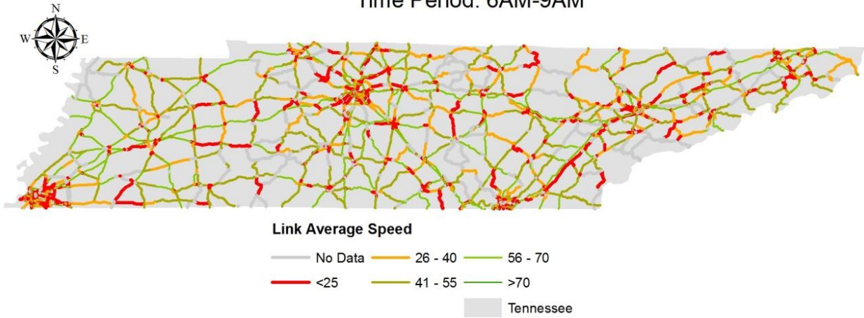
FIGURE A-10a Average Speeds, November 6 th - 8 th , AM Period.
