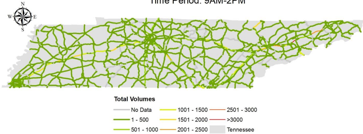
FIGURE B-17a Total Volumes, October 16 th - 18 th , AM Period
