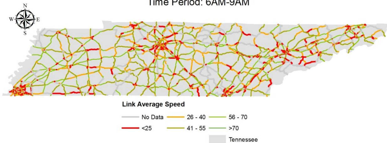
FIGURE A-5a Link Average Speeds, June 12 th - 14 th , AM Period.
