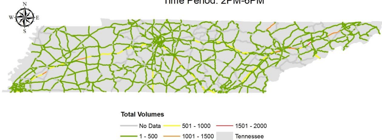
FIGURE B-1b Total Volumes, February 21 st - 23 rd , PM Period.
