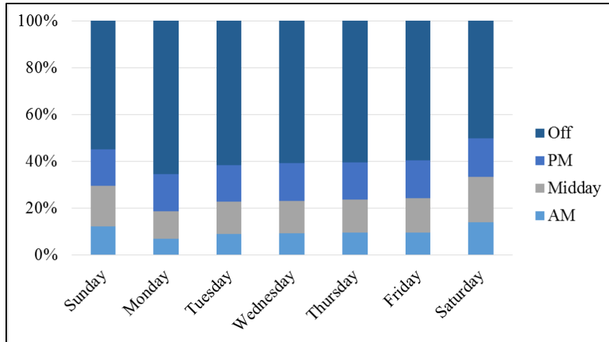
FIGURE 6 Stopped Truck Distribution by Day of the Week and Time of the Day.
