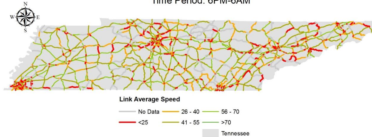
FIGURE A-2d Link Average Speeds, March 20 th - 22 nd , OP Period.
