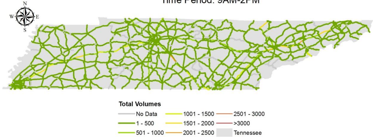
FIGURE B-16a Total Volumes, September 18 th - 20 th , MD Period.
