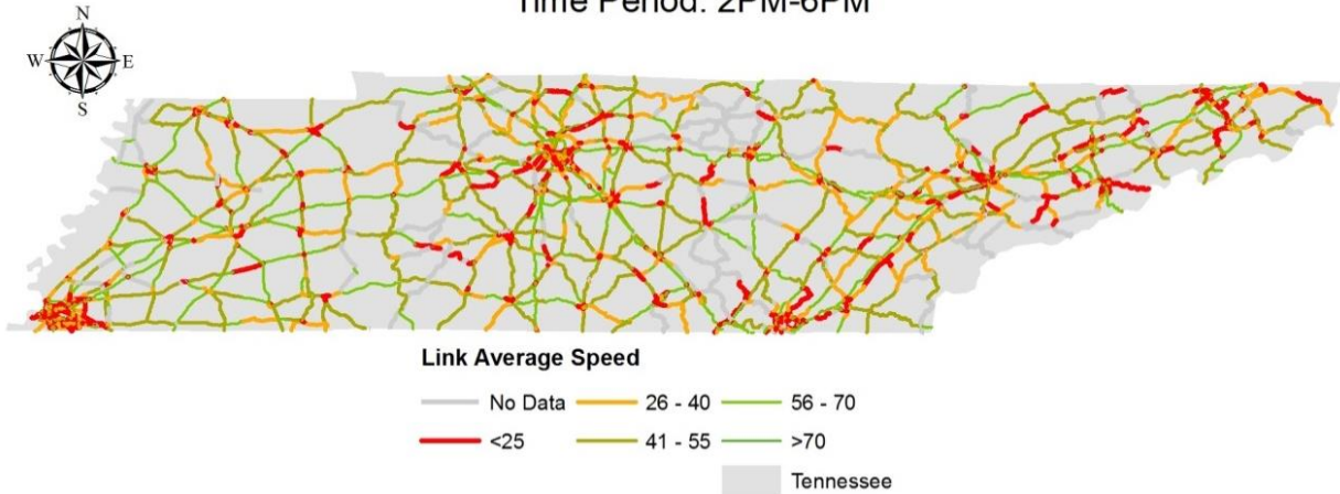
FIGURE A-3c Link Average Speeds, April 17 th - 19 th , PM Period.
