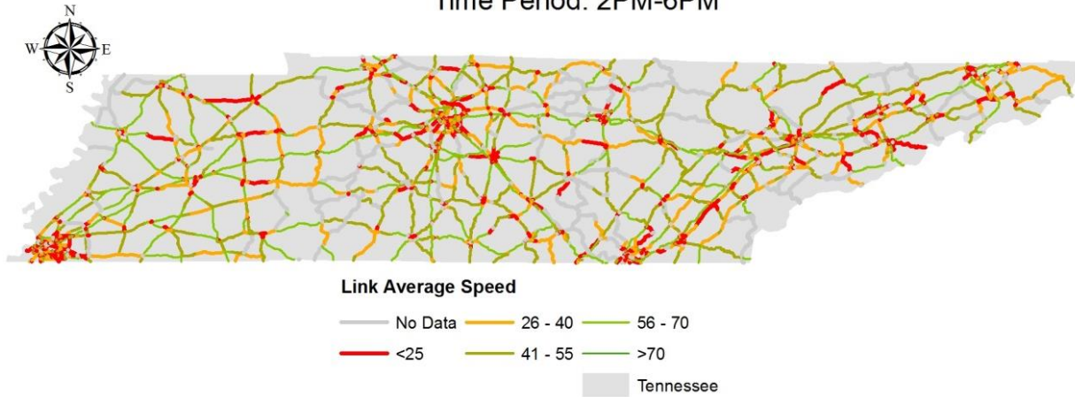
FIGURE A-2c Link Average Speeds, March 20th - 22nd, PM Period.
