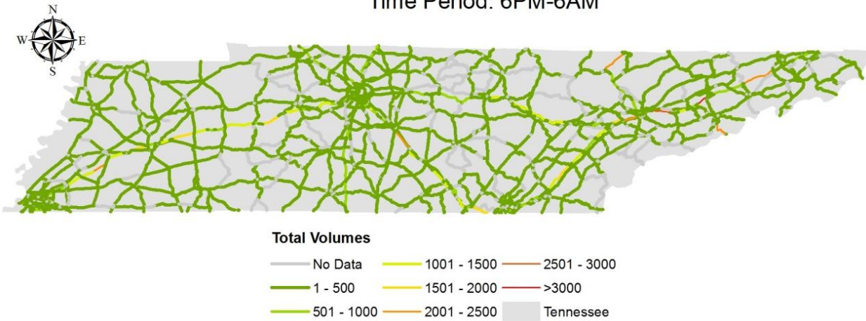
FIGURE B-2b Total Volumes, February 21 st - 23 rd , OP Period
