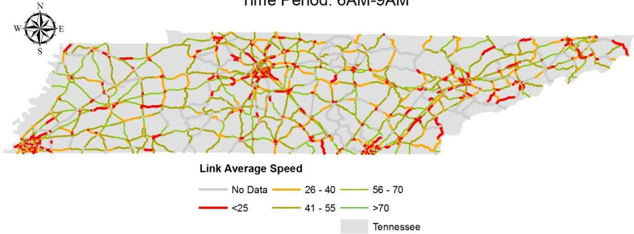
FIGURE A-6a Link Average Speeds, July 17 th - 19 th , AM Period.
