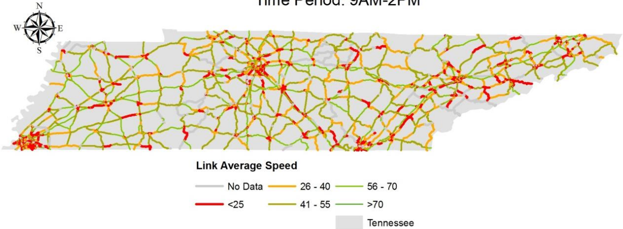
FIGURE A-1b Link Average Speeds, February 21 st – 23 rd , MD Period.
