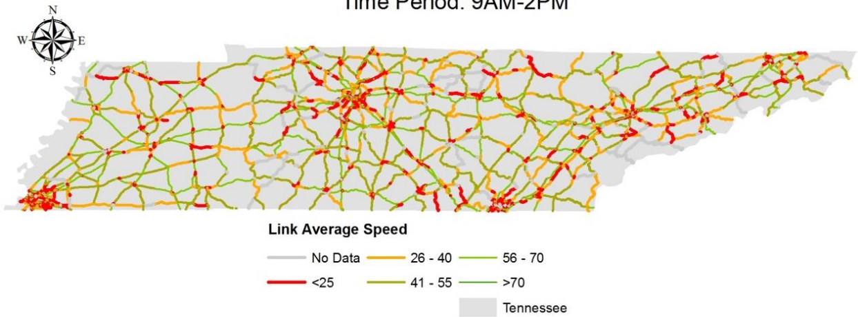
FIGURE A-2b Link Average Speeds, March 20 th - 22 nd , MD Period.
