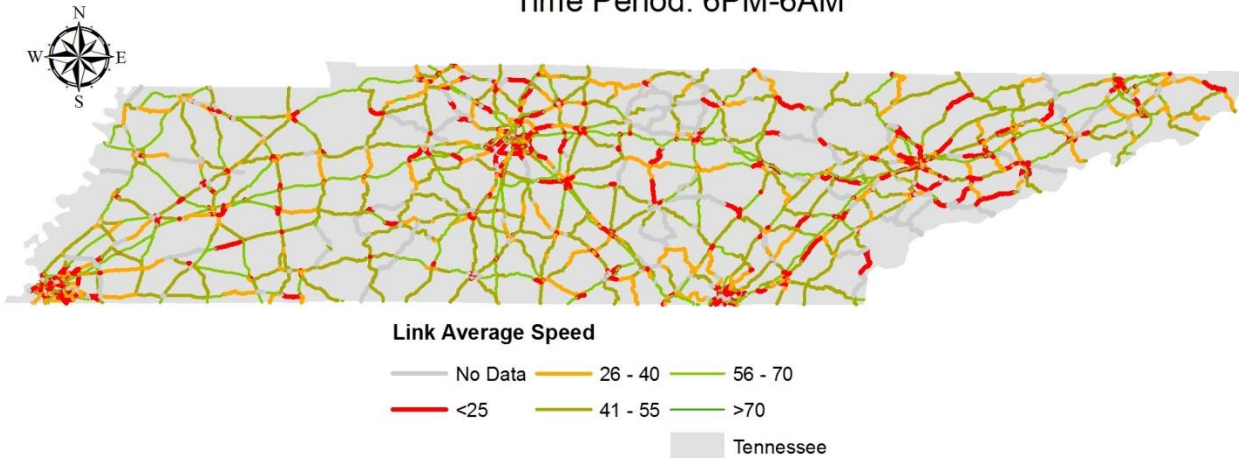
FIGURE A-10d Average Speeds, November 6 th - 8 th , OP Period.
