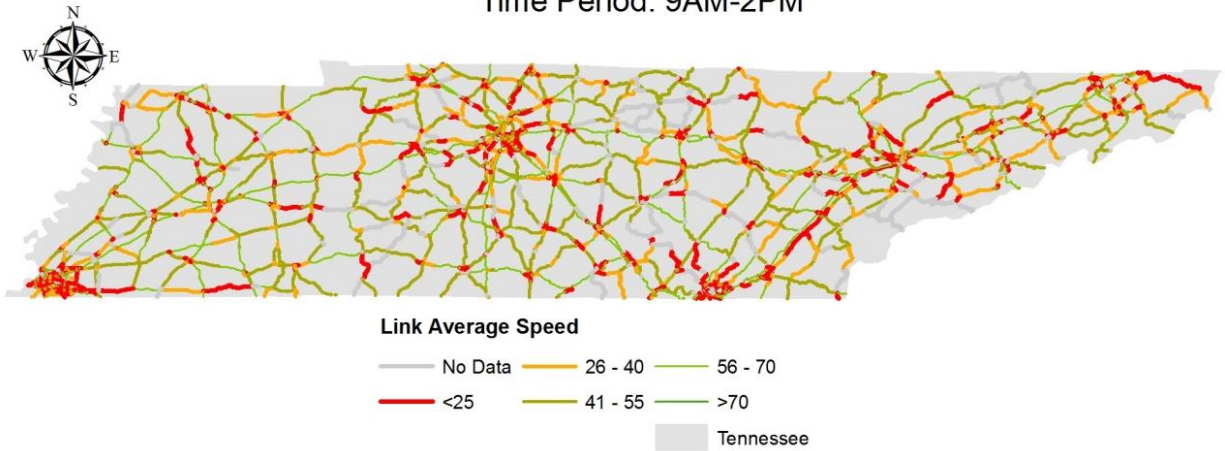
FIGURE 11b Link Average Speeds, January 3 rd – 5 th , MD Period.
