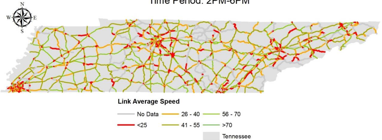
FIGURE 11c Link Average Speeds, January 3 rd – 5 th , PM Period.
