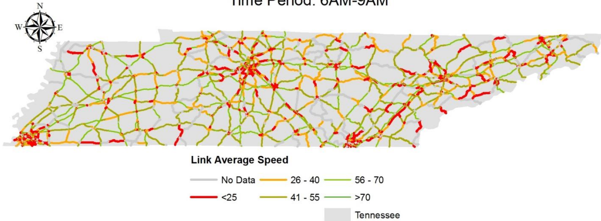
FIGURE A-4a Link Average Speeds, May 15 th - 17 th , AM Period.
