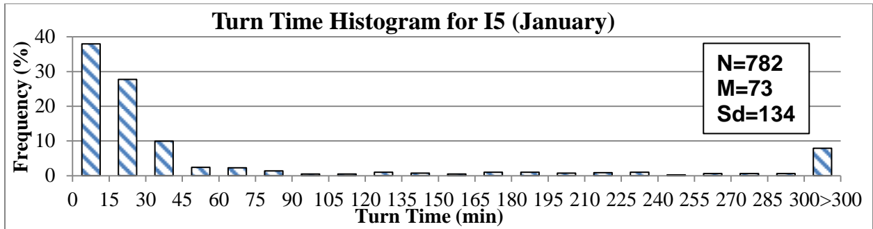
FIGURE C-1 Turn Time Histograms for Intermodal Facilities.
