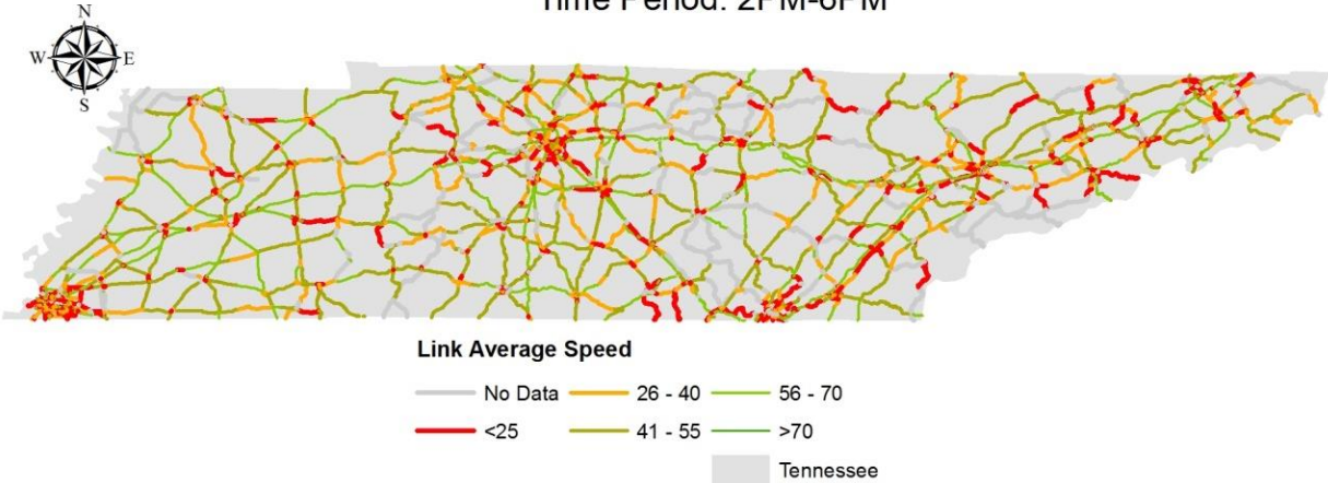
FIGURE A-9c Average Speeds, October 16 th - 18 th , PM Period.
