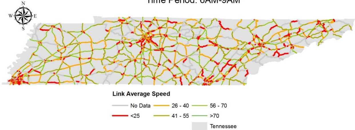
FIGURE A-1a Link Average Speeds, February 21 st – 23 rd , AM Period.
