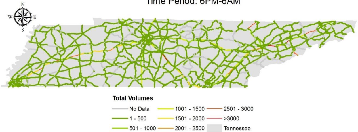
FIGURE B-20b Total Volumes, November 6 th - 8 th , OP Period.
