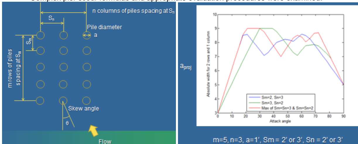
Effective pier width formulation and its variation with foundation/flow parameters
