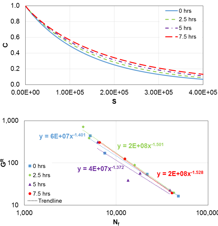
14 15 FIGURE 4 S-VECD virgin mixture results: a) damage characteristic curves and b) fatigue 16 failure criterion.
