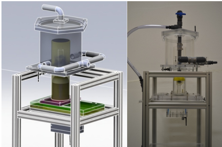
Computer rendering and photograph of the calibration device
