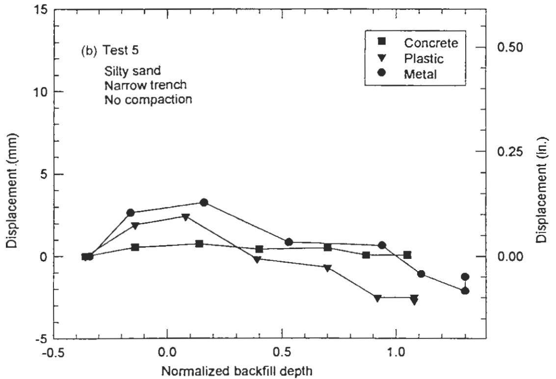
Figure 4.52 Sidefill Soil Displacement During Backfilling
