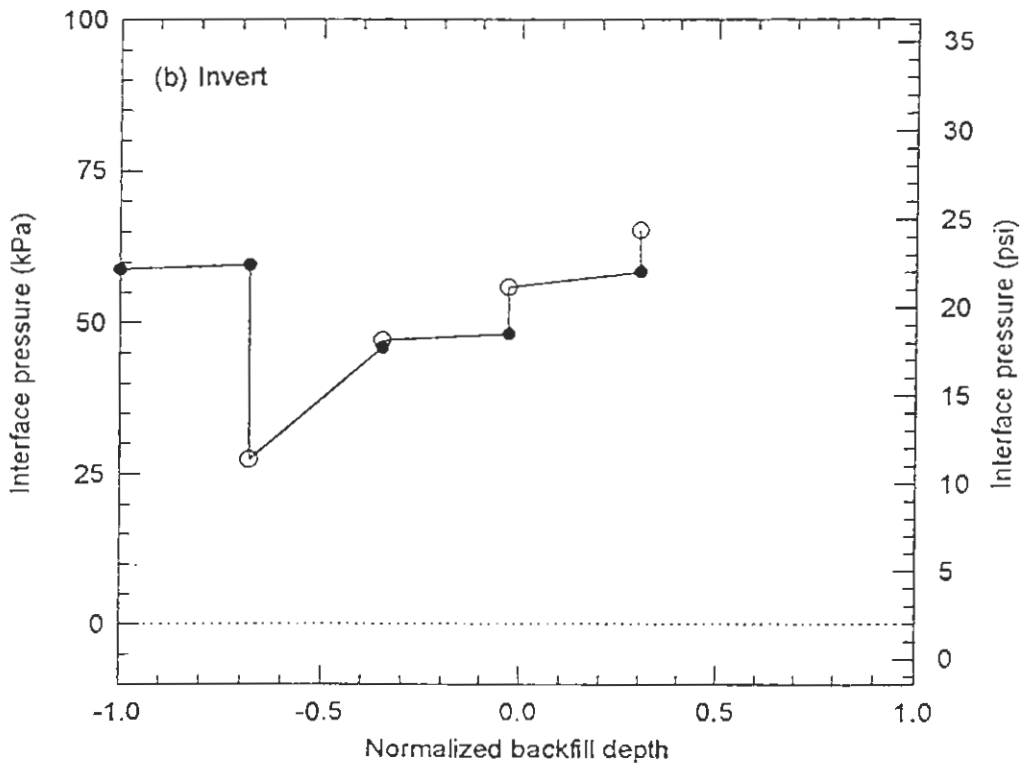
Figure 4.8 Concrete Pipe-Soil Interface Pressures (Lab Test 11)
