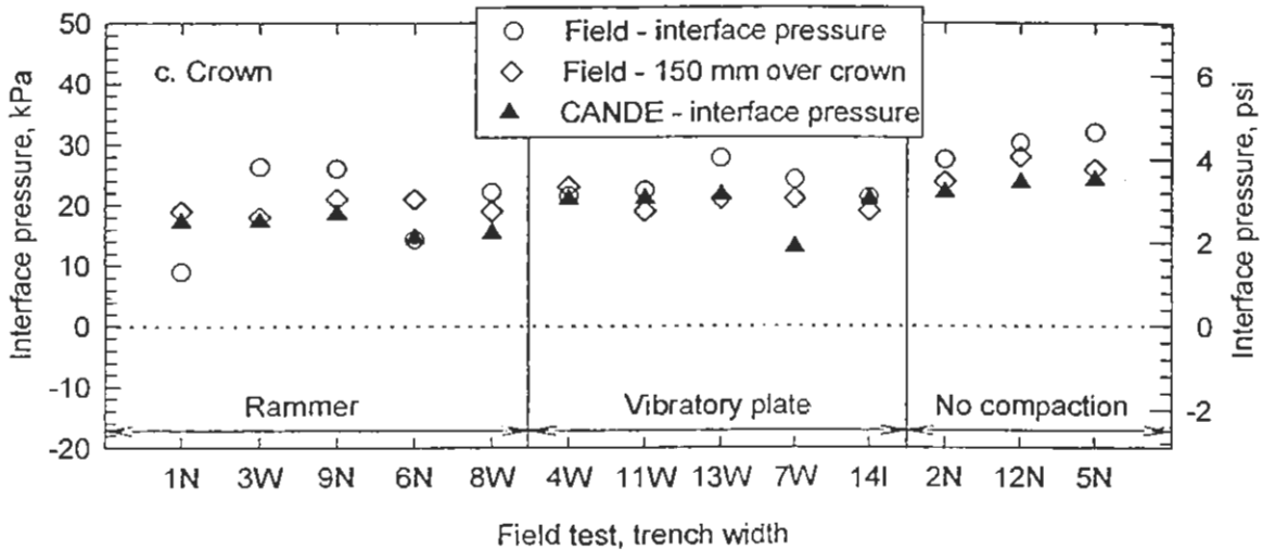
Figure 5.10 CANDE Interface Pressures Compared to Field Pressures for Concrete Pipe
