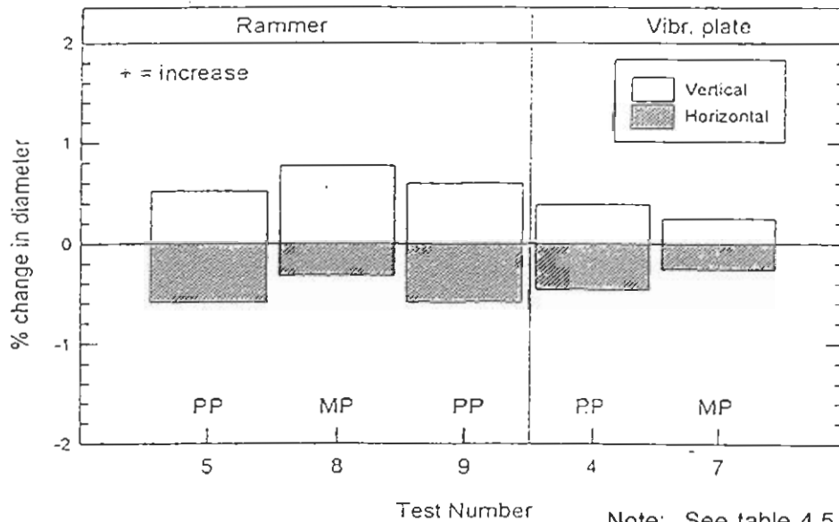
Figure 4.15 Comparison of Pipe Deflections with Pipe Type and Method of Compaction, Backfill Compacted to the Springline Lift
