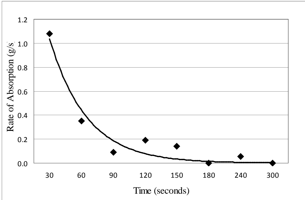
Figure 1. 8mm thick geotextile rate of water absorption
