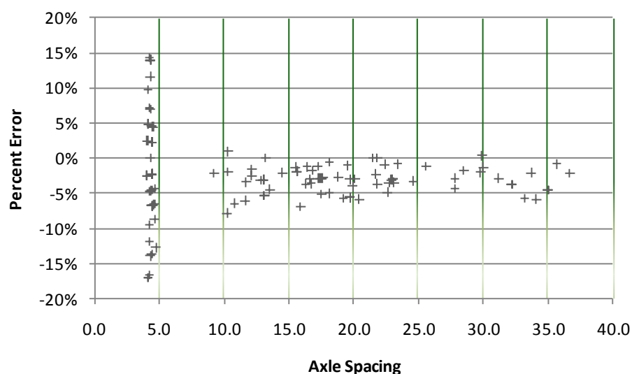
Figure 16. Percent Error of AxleLight at Various Axle Spacings
