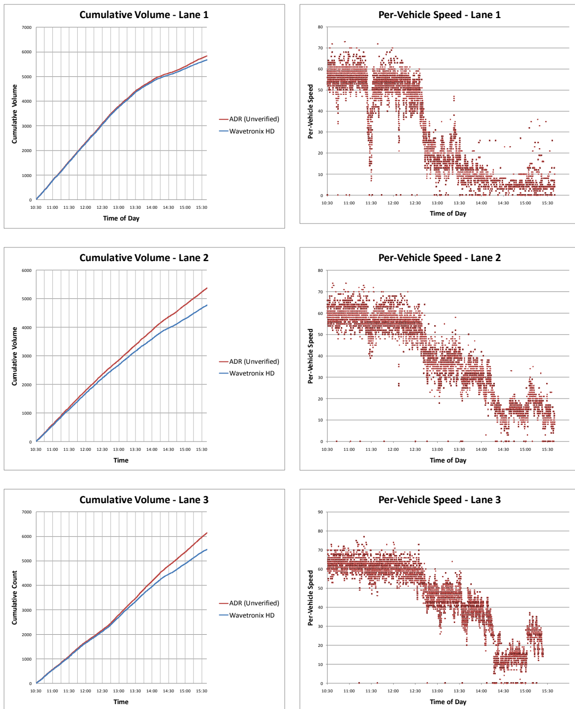
Figure 7. Wavetronix SmartSensor HD data captured on December 8, 2009 Traffic was unusually slow due to light snow conditions. Traffic undercounting in Lanes 2-3 (far two lanes) is attributed to occlusion from Lane 1 (lane nearest sensor).
