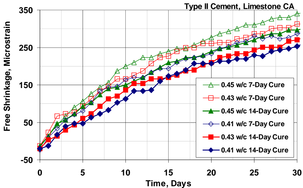
Fig. 4.5 – Free-Shrinkage Test (ASTM C 157). Program I Set 2. Average free shrinkage versus time through 30 days (drying only).
