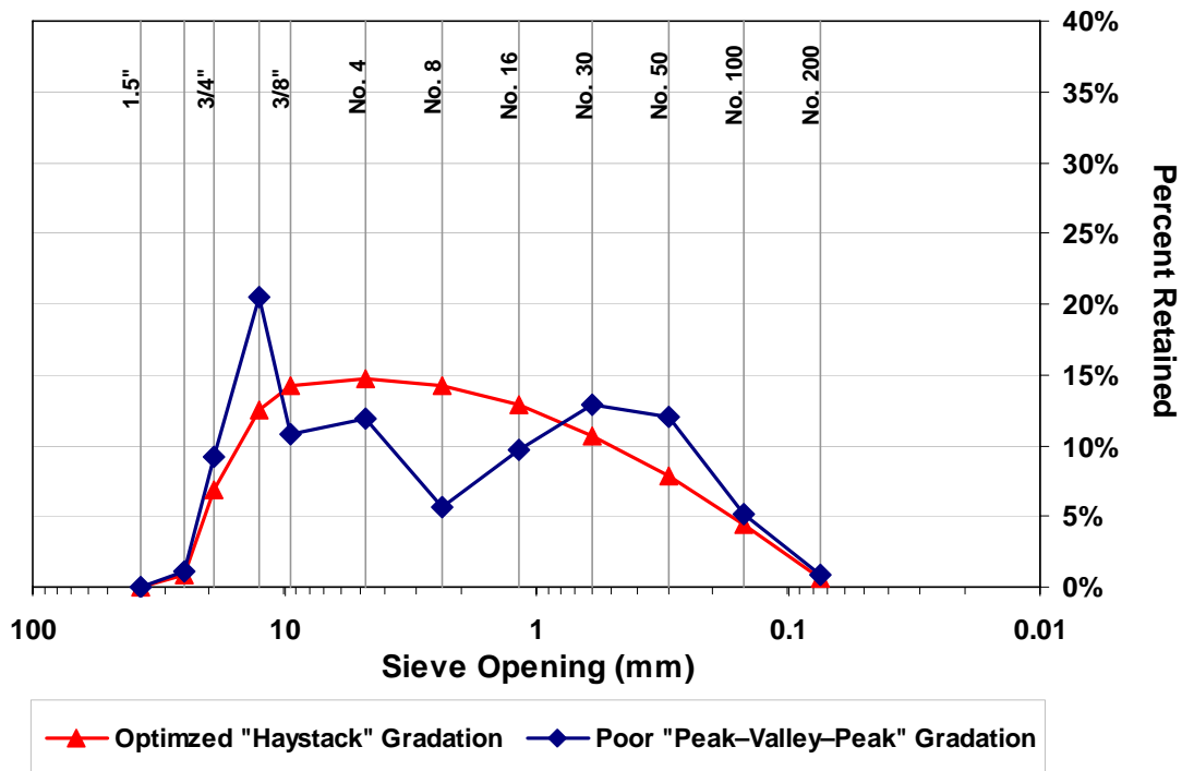
Fig. 1.1 – Percent retained chart for combined aggregates with an optimized “haystack” gradation and a poor “peak–valley–peak” gradation.
