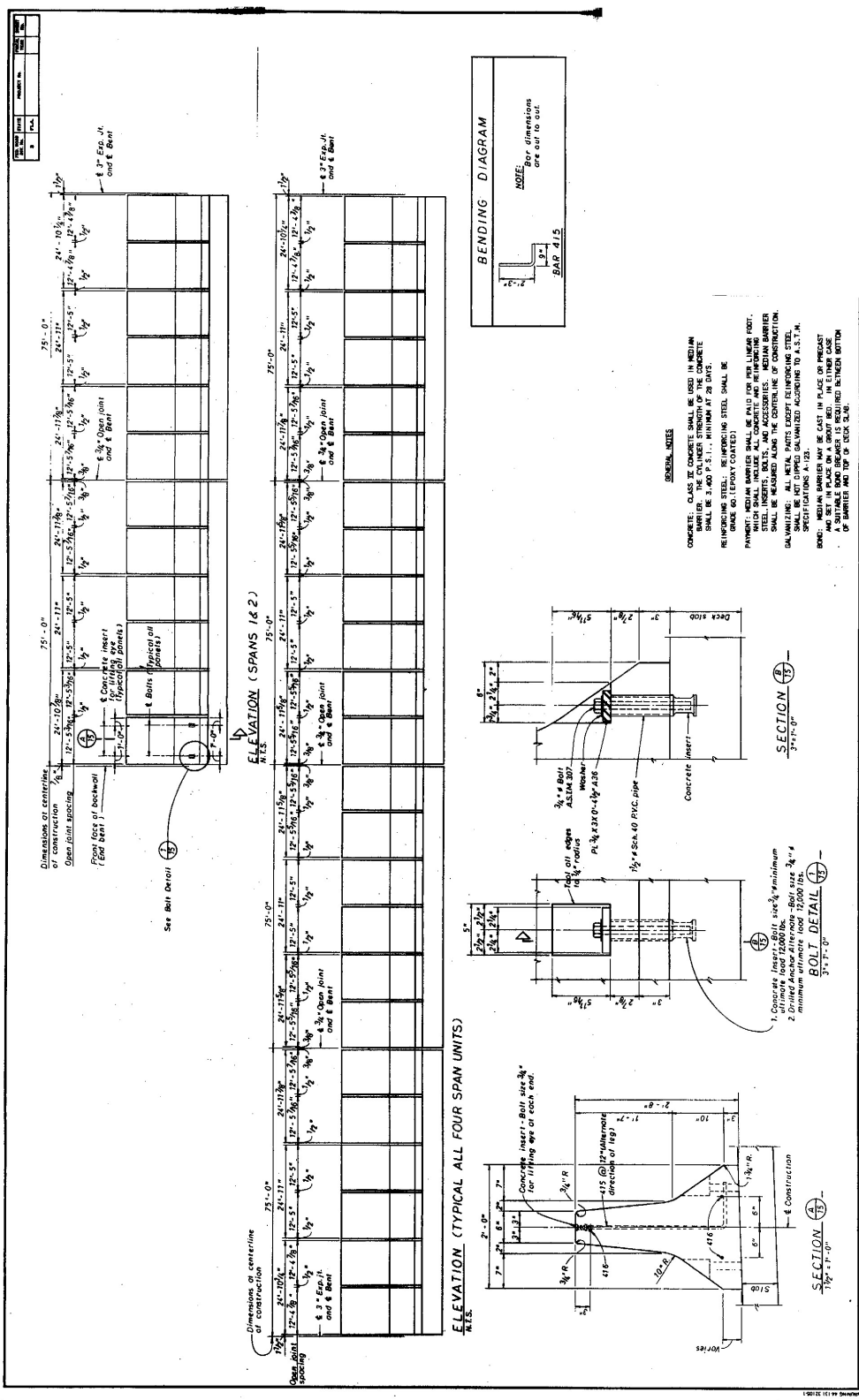
Figure 3. Median Barrier Details
