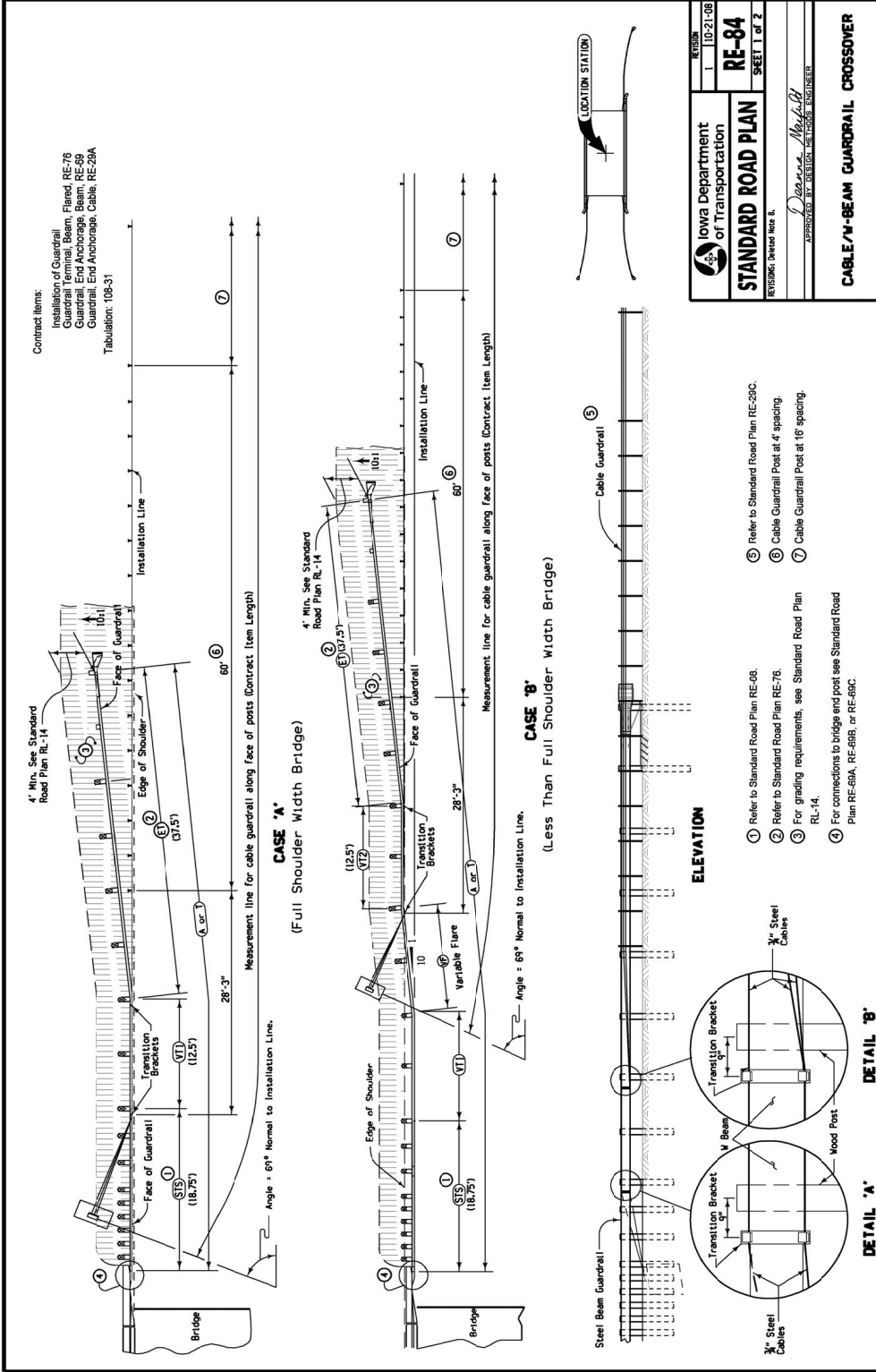
Figure 4. Cable to W-Beam Transition
