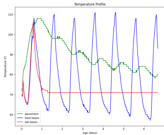
Figure 3 Temperature profile
