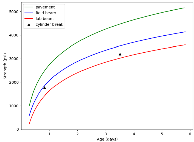
Figure 2 Sensing results versus cylinder break
