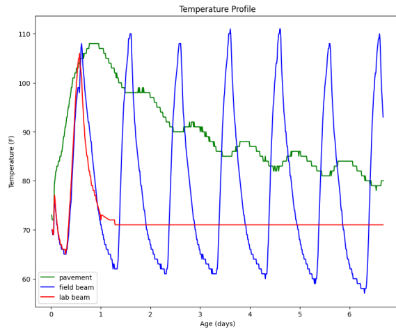
Figure 3 Temperature profile
