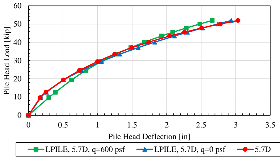
Figure 6-10. Comparison of measured pile head load versus deflection curve for the 5.7D square pile with curves computed using LPILE assuming no surcharge and 600 psf surcharge.
