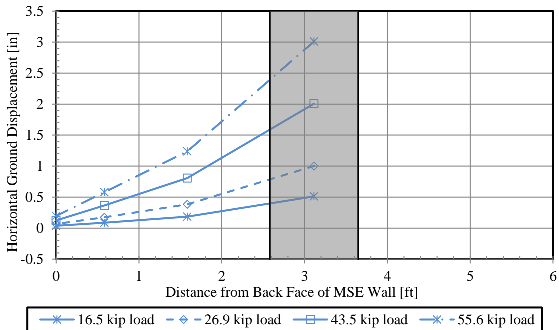
Figure E.2-3: Horizontal ground displacement at several load levels for 2.9D test.
