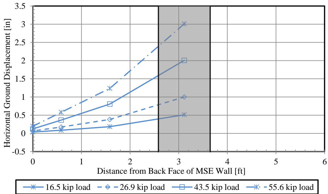
Figure 6-23: Horizontal ground displacement for 2.9D test at several pile head load levels.
