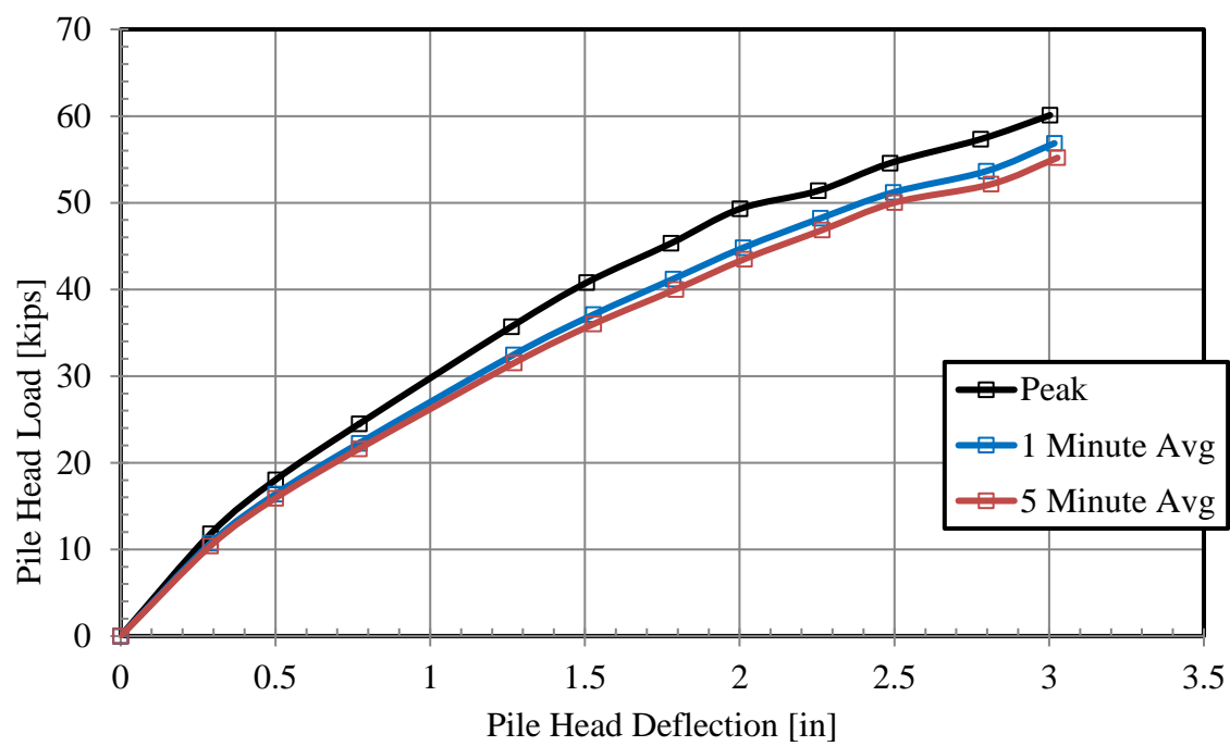
Figure D.2-4. Load-deflection curves for 3.9D test.
