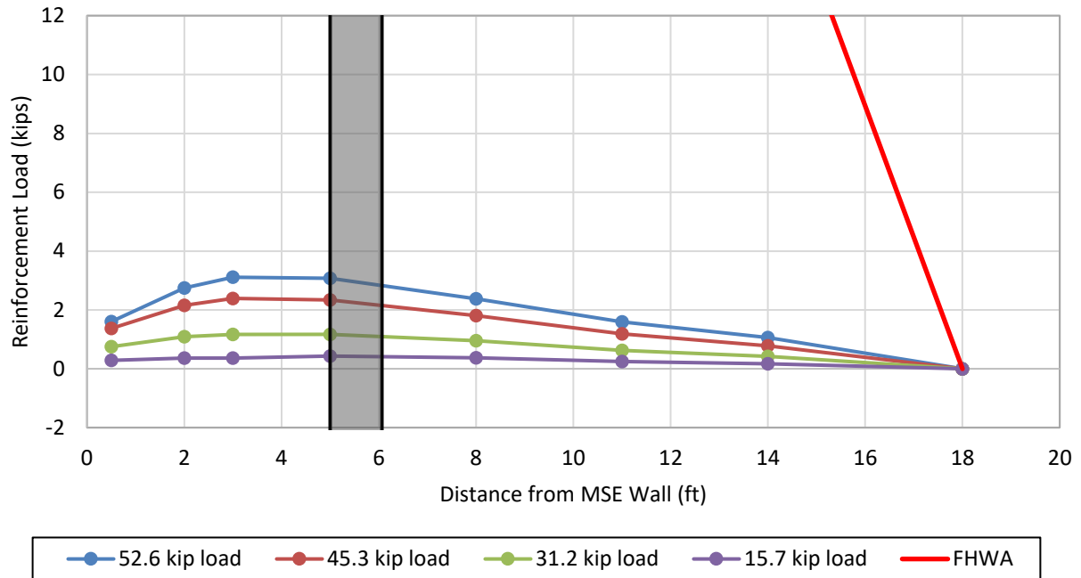
Figure F.1-7: Induced loads in the soil reinforcement at different pile head loads relative to distance from the back of the MSE wall (5.2D pile, layer L4, 39 in. transverse spacing).
