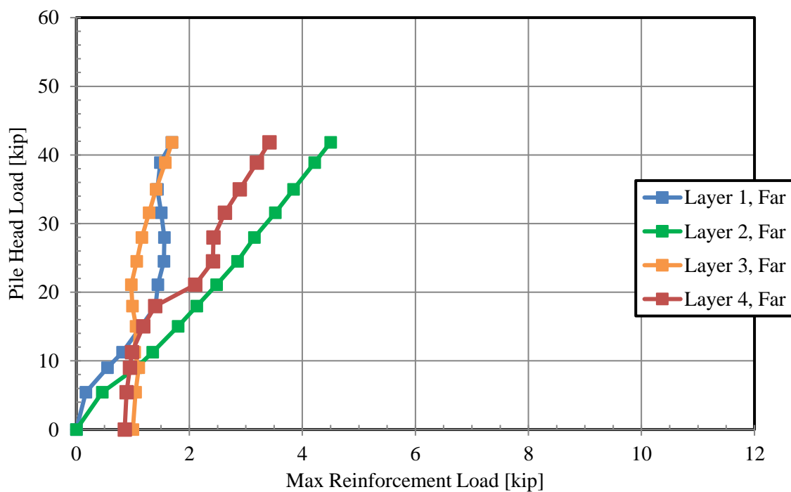
Figure 6-6: Max tensile force in far soil reinforcement at each pile head load for 1.7D test.
