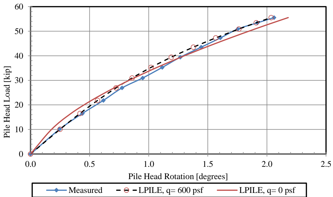
Figure 8-7: Comparison of pile head load versus rotation curves computed by LPILE to measured pile head load versus rotation curves for the 2.9D test.
