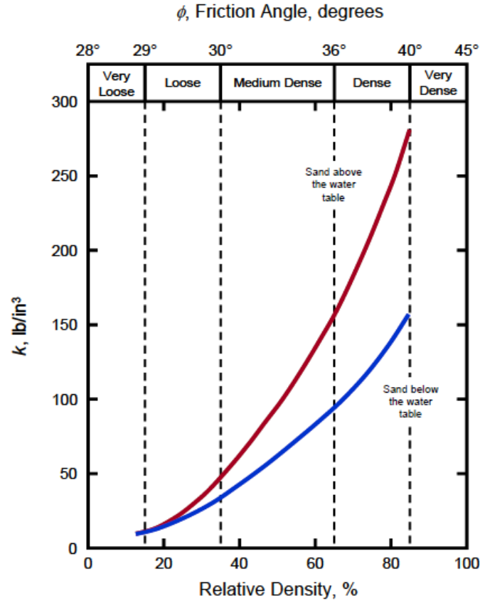
Figure 2-9: Soil modulus reaction based on friction angle or relative density of soil (API, 1982).
