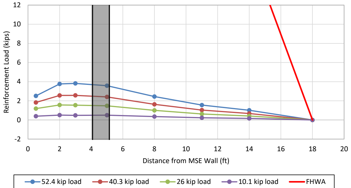
Figure F.1-15: Induced loads in the soil reinforcement at different pile head loads relative to distance from the back of the MSE wall (4.3D pile, layer L4, 34 in. transverse spacing).
