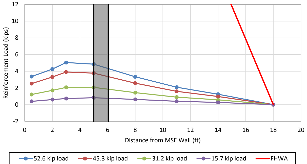
Figure F.1-5: Induced loads in the soil reinforcement at different pile head loads relative to distance from the back of the MSE wall (5.2D pile, layer L3, 46 in. transverse spacing).
