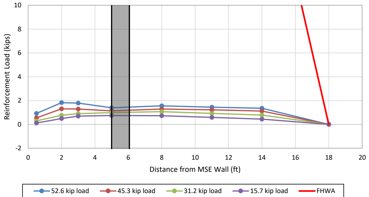
Figure F.1-1: Induced loads in the soil reinforcement at different pile head loads relative to distance from the back of the MSE wall (5.2D pile, layer L1, 46.5 in. transverse spacing).
