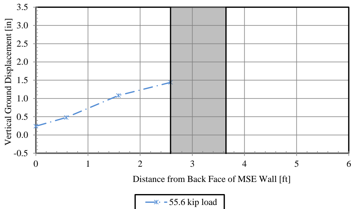
Figure E.2-7: Vertical ground displacement at peak pile load for 2.9D test.
