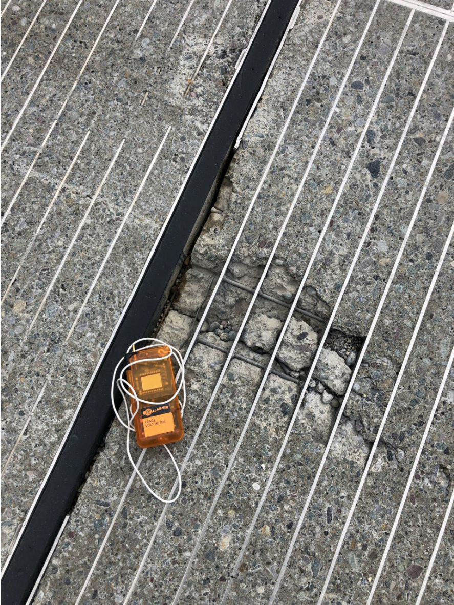
Figure 37: Crumbling concrete at the western electrified barrier, presumably associated with a change in slope after the bridge abutment settled (image Samantha Getty).
